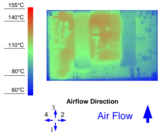
Figure 8. Thermal Image for Airflow Direction 3 (43A output, 55°C ambient, 200 LFM, typical Vin, open frame, soldered interface)
