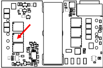
Figure 15. Temperature Monitoring Locations
