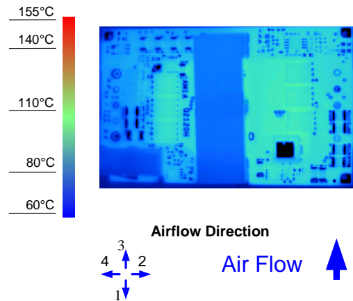
Figure 8. Thermal Image for Airflow Direction 3 (12A output, 55°C ambient, 200 LFM, typical Vin, open frame, unit soldered onto a fixture board)
