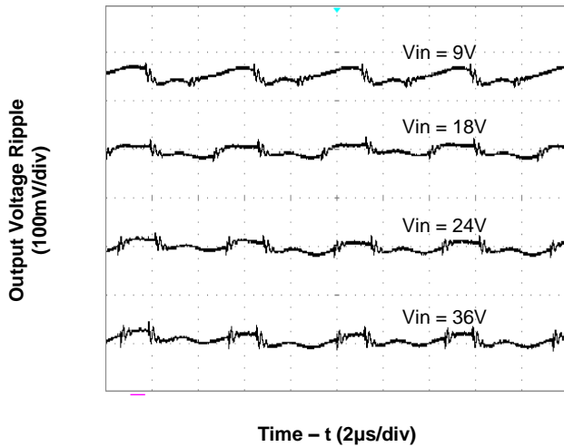
Figure 3. Output Ripple Voltage at Full Load
