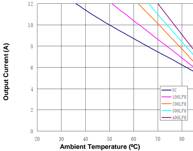
Figure 7. Current Derating Curve for Airflow Direction 3 (Ref. Fig. 8 for Airflow Direction; typical Vin, open frame, unit soldered onto a fixture board)
