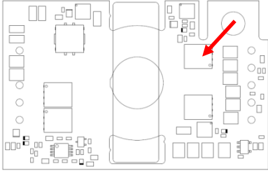
Figure 18. Temperature Monitoring Locations
