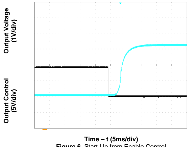
Figure 6. Start-Up from Enable Control (typical Vin and full load)
