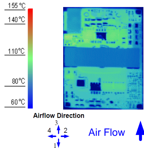
Figure 12. Thermal Image for Airflow Direction 3 (30A output, 55°C ambient, 200 LFM, typical Vin, open frame, soldered interface)
