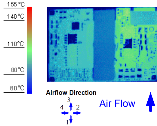
Figure 10. Thermal Image for Airflow Direction 3 (30A output, 55°C ambient, 200 LFM, typical Vin, open frame, soldered interface)
