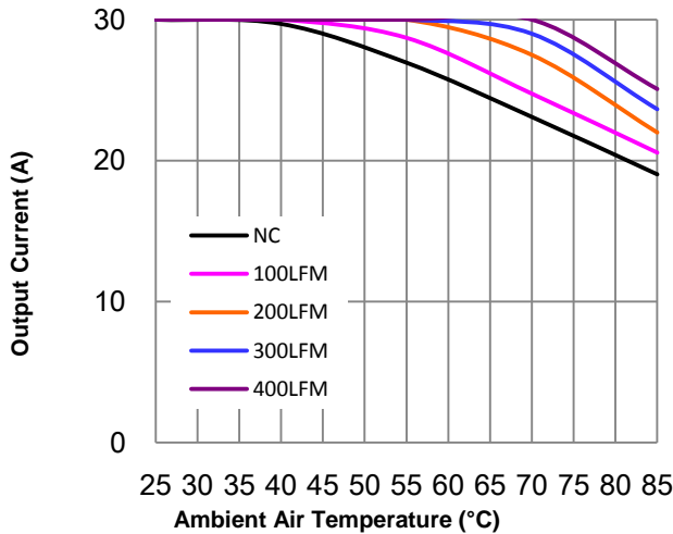
Figure 11. Current Derating Curve for Airflow Direction 3 (Ref. Fig.12 for Airflow Direction; typical Vin, open frame, soldered interface)
