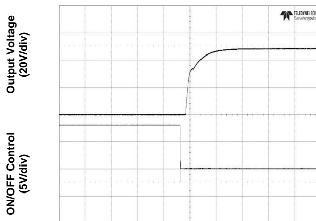
Figure 6. Start-Up from Enable Control (typical Vin, zero load)
