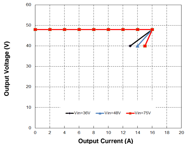
Figure 4. Output Characteristics (no parallel version)
