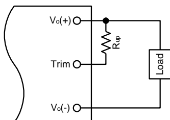
Figure 16. Circuit to Increase Output Voltage Set Point
