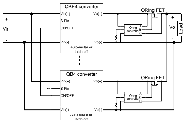
Figure 20. The connection diagram of parallel version auto-restart/latch-off QBE4 converters with ORing devices
