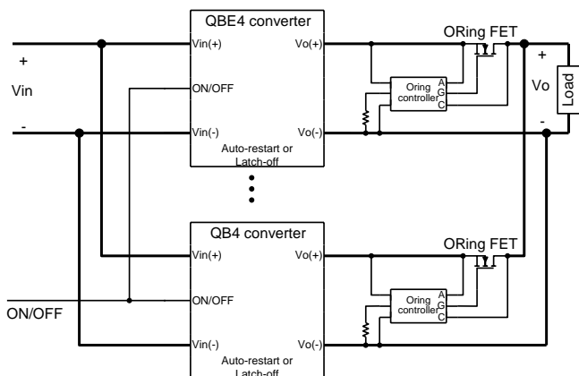
Figure 19. The connection diagram of QBE4 converters for N+1 application and/or power expansion
