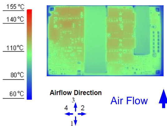
Figure 10. Thermal Image for Airflow Direction 3 (9A output, 55°C ambient, 200 LFM, typical Vin, open frame)
