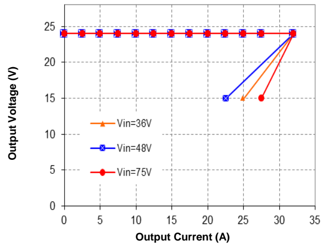
Figure 4. Output Characteristics (no parallel version)
