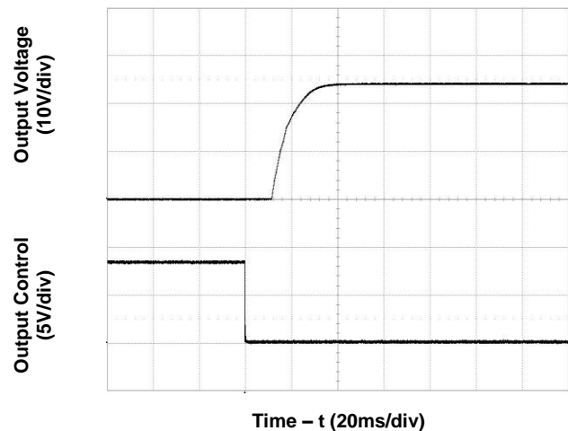
Figure 6. Start-Up from Enable Control (typical Vin, zero load)
