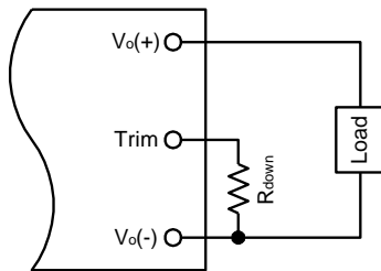
Figure 15. Circuit to Decrease Output Voltage
