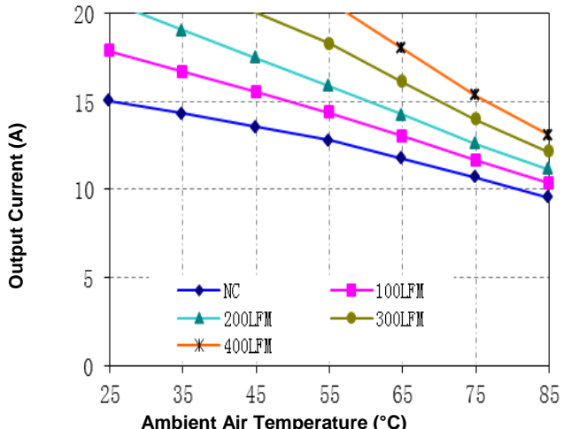
Figure 11. Current Derating Curve With Baseplate
