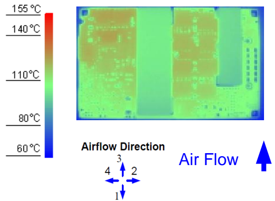
Figure 10. Thermal Image for Airflow Direction 3 (14A output, 55°C ambient, 200 LFM, typical Vin, open frame)
