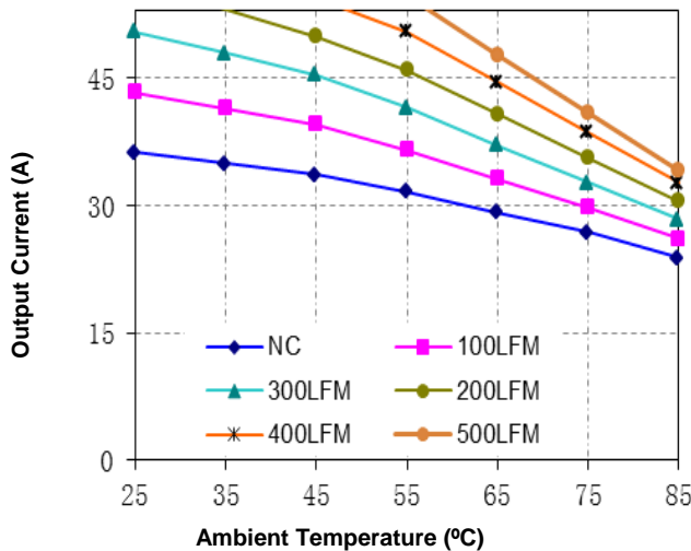
Figure 11. Derating Curve for Airflow Direction 3 (Ref. Figure 10 for Airflow Direction; Vin = 48V; unit with baseplate)
