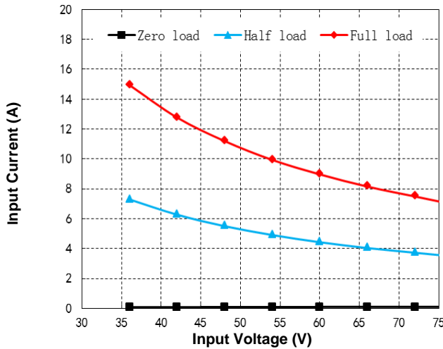
Figure 3. Input Characteristic (25°C)
