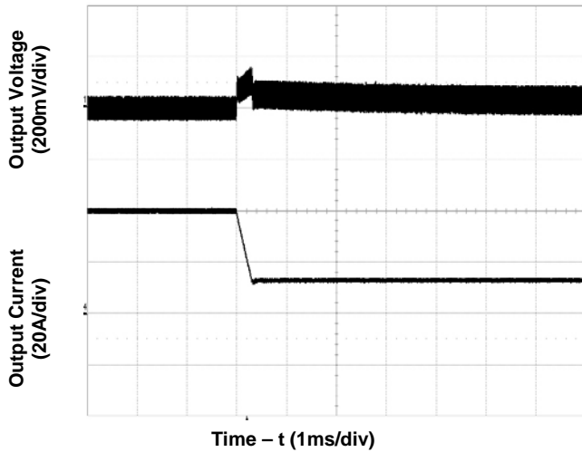
Figure 7. Transient Load Response (typical Vin, load current steps from 50% to 25% at a slew rate 0.1A/μs)
