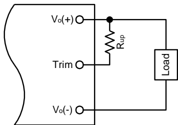
Figure 15. Circuit to Increase Output Voltage
