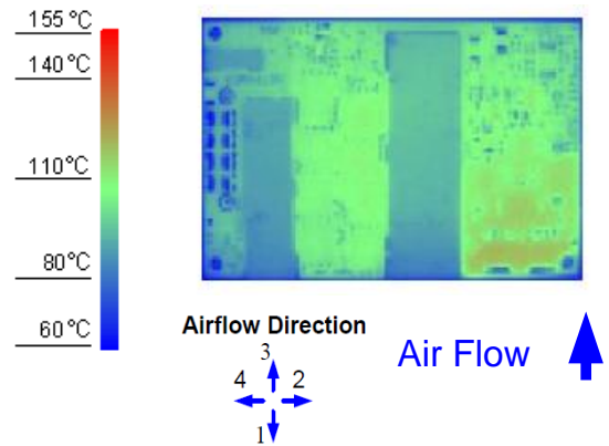
Figure 10. Thermal Image for Airflow Direction 3 (33A output, 55°C ambient, 200 LFM, typical Vin, open frame, soldered interface)
