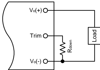
Figure 14. Circuit to Decrease Output Voltage
