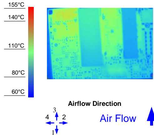
Figure 8. Thermal Image for Airflow Direction 3 (7A output, 55°C ambient, 200 LFM, typical Vin, open frame, unit soldered onto a fixture board)
