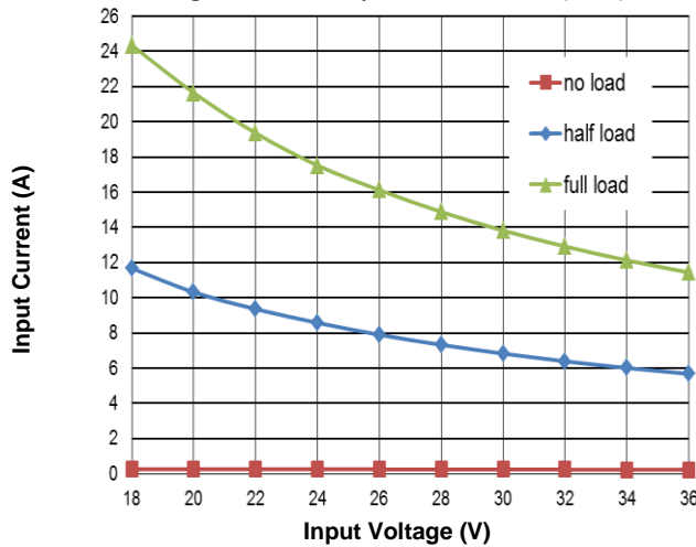
Figure 3. Input Characteristics
