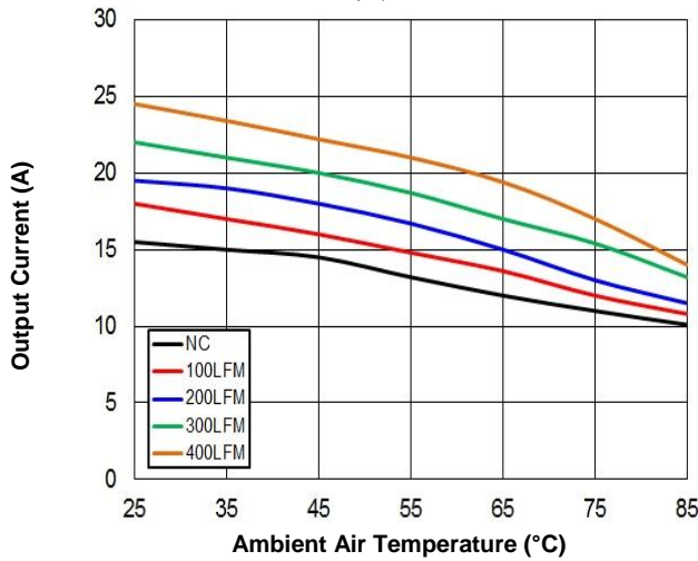
Figure 8. Current Derating Curve for Airflow Direction 3 (Ref. Fig. 9 for Airflow Direction; typical V_{in} , open frame, unit soldered onto a fixture board)
