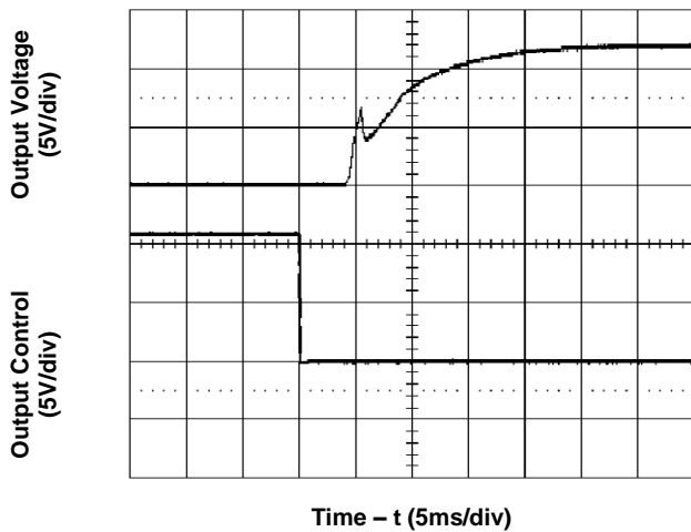
Figure 5. Start-Up from Enable Control (typical V_{in} , full load, tested in CR mode)
