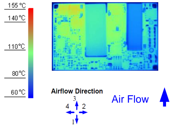
Figure 9. Thermal Image for Airflow Direction 3 (17A output, 55^{\circ}C ambient, 200 LFM, typical V_{in} , open frame, unit soldered onto a fixture board)
