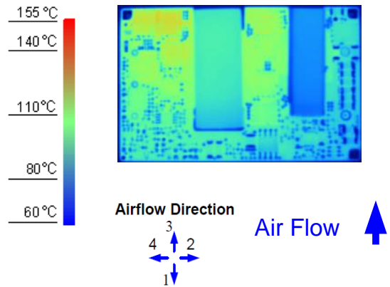
Figure 9. Thermal Image for Airflow Direction 3 (15.5A output, 55°C ambient, 200 LFM, typical V_{in} , open frame, unit soldered onto a fixture board)
