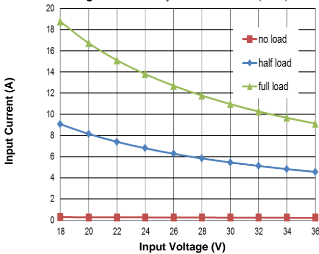
Figure 3. Input Characteristics
