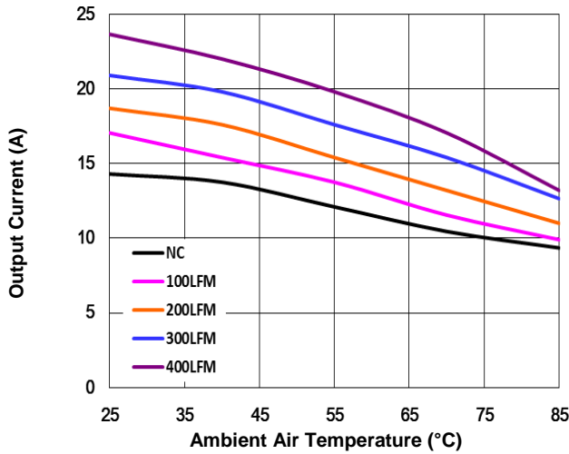
Figure 8. Current Derating Curve for Airflow Direction 3 (Ref. Fig. 9 for Airflow Direction; typical V_{in} , open frame, unit soldered onto a fixture board)
