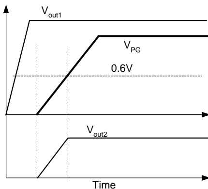
Figure 29. Sequential Startup Waveforms
