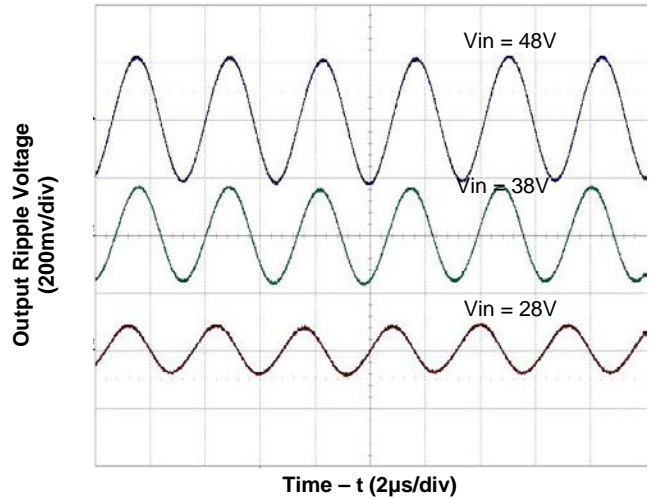
Figure 2. Output Ripple Voltage ( V_o=24V ; I_o=13A ; C_{o,ex}=470\mu F )
