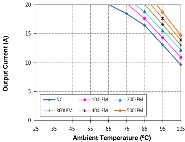
Figure 14a. Derating with Open-frame ( V_{in}=24V and V_o=3.3V )
