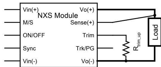
Figure 23. Circuit Configuration for Output Voltage Trim Up
