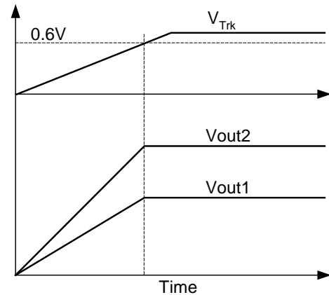
Figure 25. Ratio-metric Tracking Waveforms
