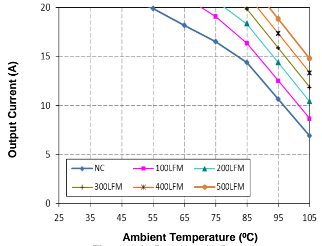
Figure 17b. Derating with Baseplate ( V_{in}=18V and V_o=12V )
