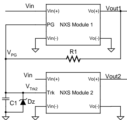
Figure 28. Circuit Configuration for Sequential Startup
