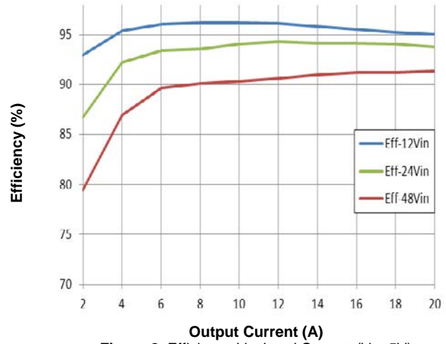
Figure 8. Efficiency Vs. Load Current (Vo=5V)
