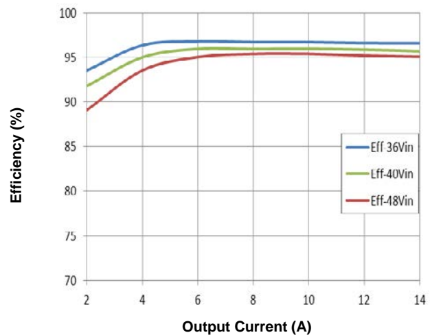
Figure 12. Efficiency Vs. Load Current (Vo=24V)
