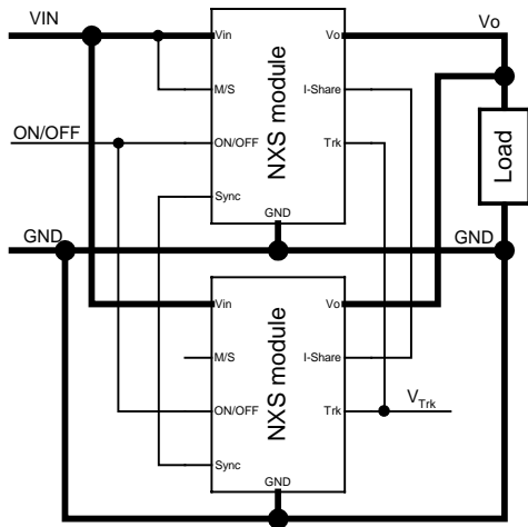
Figure 30. Circuit Configuration for Active Load Sharing
