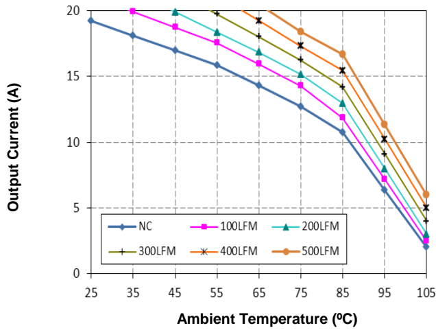
Figure 17a. Derating with Open-frame ( V_{in}=18V and V_o=12V )
