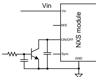
Figure 21. Open Collector Enable Circuit
