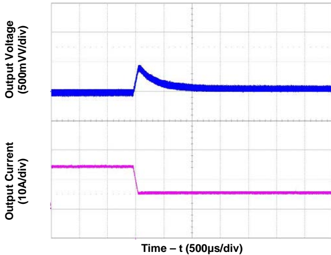
Figure 3. Transient Load Response at V_o=12V ( V_{in}=24V ; I_o=15A \rightarrow 5A @ 0.1A/\mu s ; C_{o,ex}=470\mu F )
