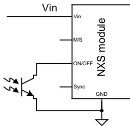
Figure 20. Opto-coupler Enable Circuit
