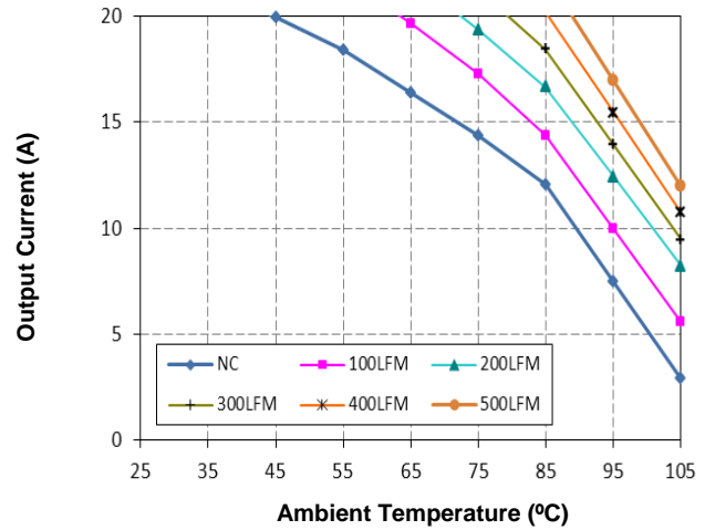
Figure 14b. Derating with Baseplate ( V_{in}=24V and V_o=3.3V )
