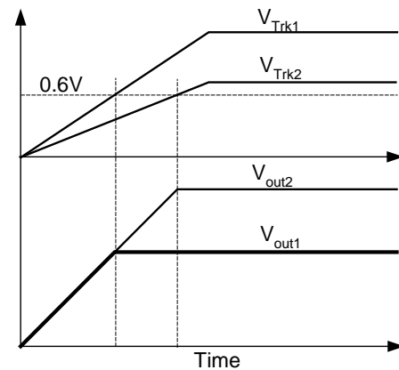
Figure 27. Simultaneous Tracking Waveforms
