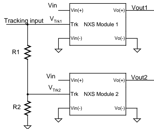
Figure 26. Circuit Configuration for Simultaneous Tracking
