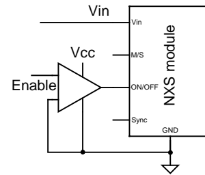
Figure 22. Direct Logic Drive
