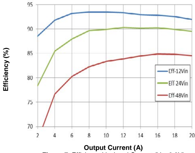
Figure 7. Efficiency Vs. Load Current (Vo=3.3V)
