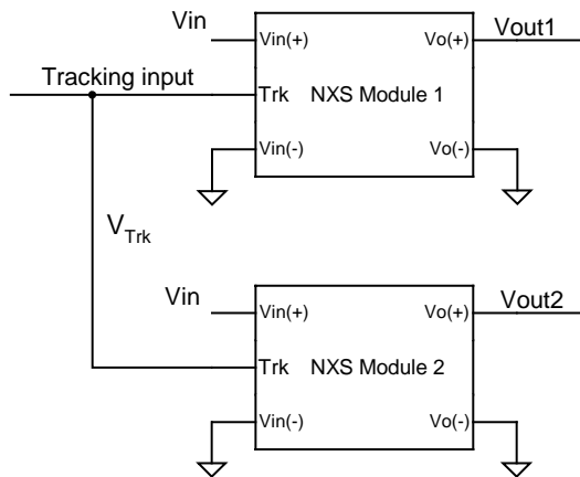
Figure 24. Circuit Configuration for Ratio-metric Tracking
