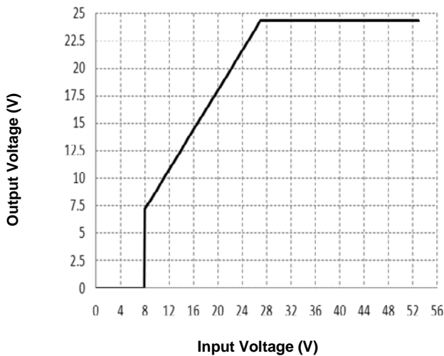
Figure 5. Output vs. Input Operating Range
