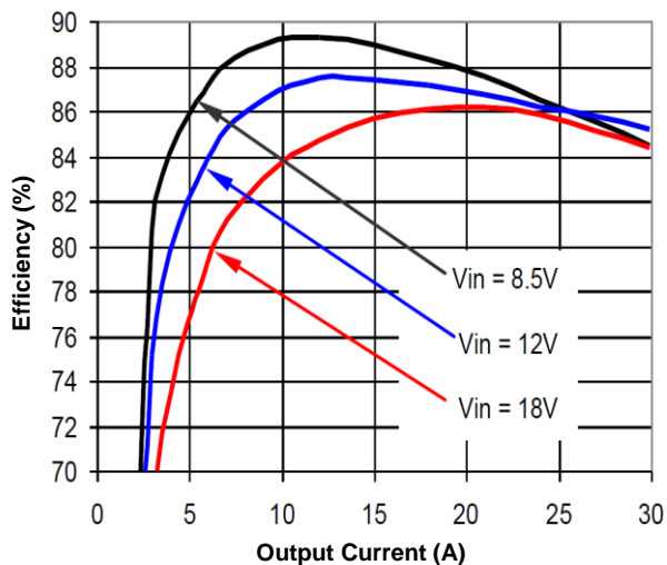
Figure 2(a). Efficiency vs. Load Current (25°C)
