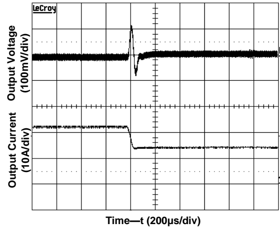
Figure 4(f). Transient Response to Load Current (Input voltage 12V ,75% I_{o,max} to 50% I_{o,max} )
