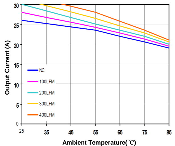
Figure 4(b). Current Derating Curve( V_{in} = 12V open frame)
