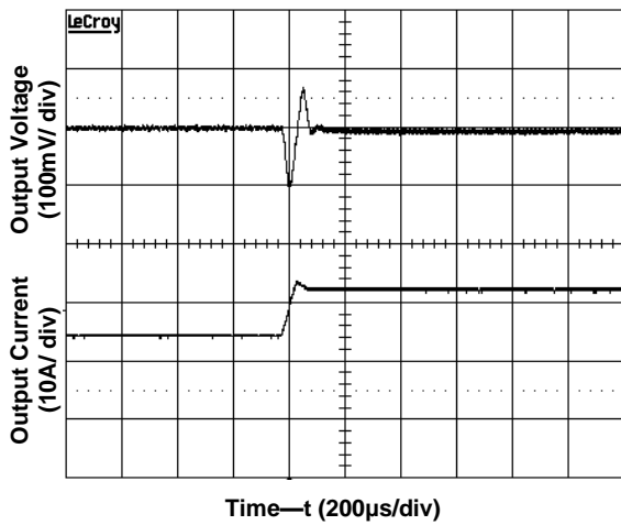
Figure 1(e). Transient Response to Load Current (Input voltage 12V, 50% I_{o,max} to 75% I_{o,max} )
