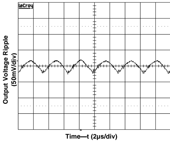
Figure 4(c). Output Ripple Voltage (Input voltage 12V ,Output Current I_{o,max} )
