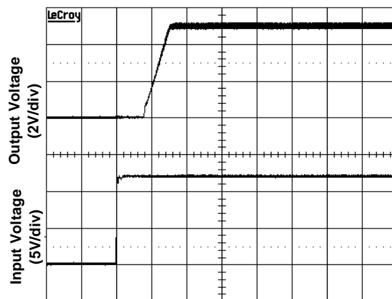
Figure 6(d). Start-up from Application of Input Voltage (Input voltage 12V, Output current I_{o,max} )
