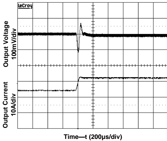
Figure 3(e). Transient Response to Load Current (Input voltage 12V ,50% I_{o,max} to 75% I_{o,max} )
