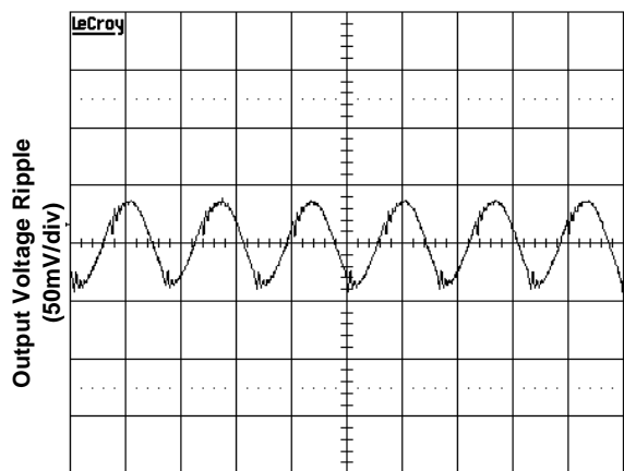
Figure 6(c). Output Ripple Voltage (Input voltage 12V, Output Current I_{o,max} )
