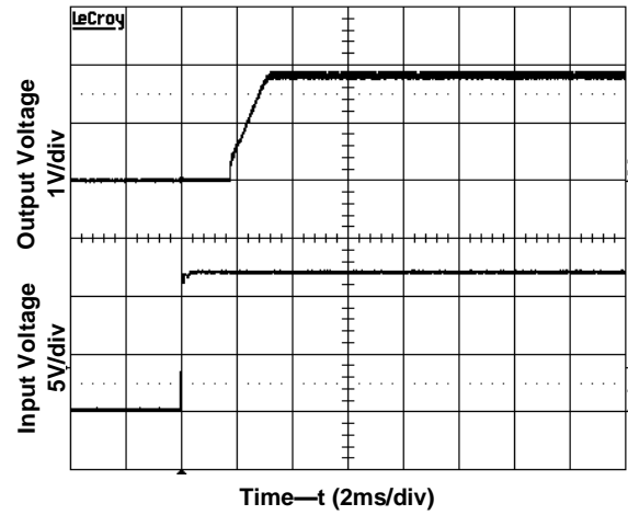
Figure 3(d). Start-up from Application of Input Voltage (Input voltage 12V, Output current I_{o,max} )
