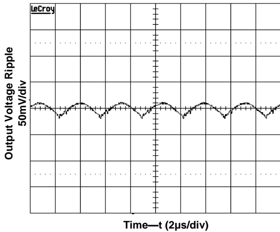
Figure 3(c). Output Ripple Voltage (Input voltage 12V ,Output Current I_{o,max} )
