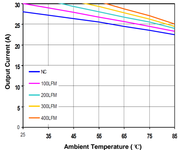
Figure 2(b). Current Derating Curve ( V_{in}=12V open frame)
