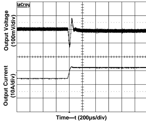
Figure 4(e). Transient Response to Load Current (Input voltage 12V ,50% I_{o,max} to 75% I_{o,max} )
