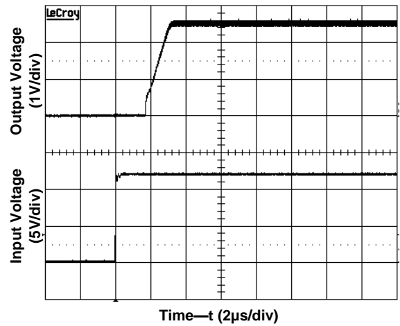
Figure 4(d). Start-up from Application of Input Voltage (Input voltage 12V, Output current I_{o,max} )
