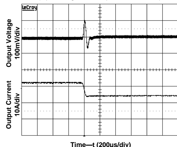
Figure 3(f). Transient Response to Load Current (Input voltage 12V ,75% I_{o,max} to 50% I_{o,max} )
