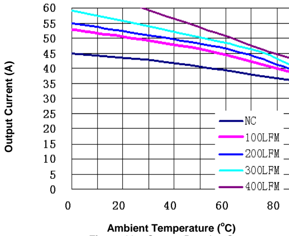
Figure 10c. Current Derating Curve ( V_{in}=12V , V_o=1.2V , open frame)
