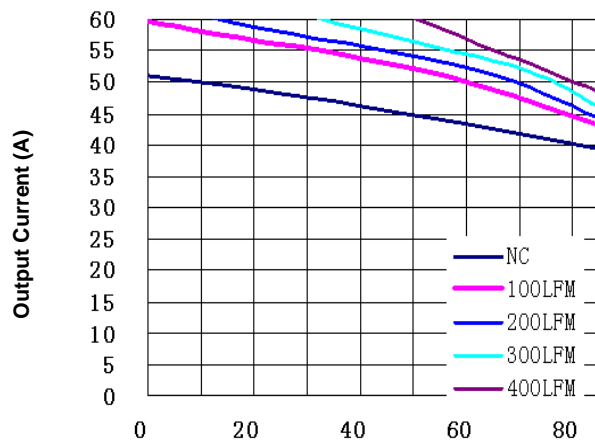
Figure 10b. Current Derating Curve (Vin=12V, Vo=1.0V, open frame)
