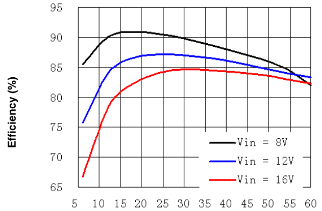
Figure 1b. Efficiency vs. Load Current (25°C, V_o=1.0V )
