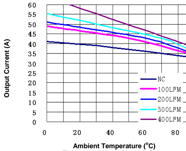
Figure 10d. Current Derating Curve ( V_{in}=12V , V_o=1.5V , open frame)
