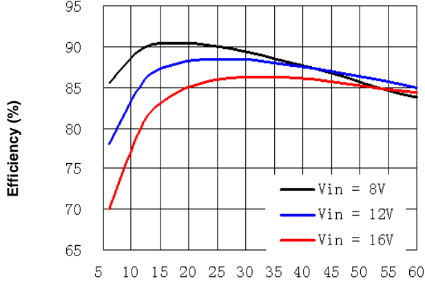
Figure 1c. Efficiency vs. Load Current (25°C, V_o=1.2V )
