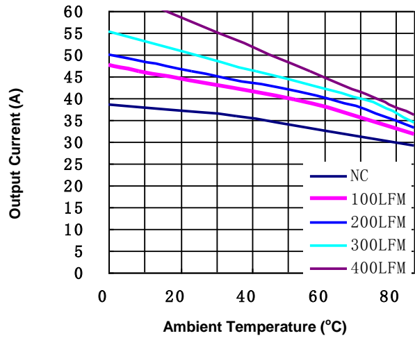
Figure 10f. Current Derating Curve ( V_{in}=12V , V_o=2.5V , open frame)
