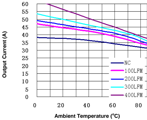
Figure 10e. Current Derating Curve ( V_{in}=12V , V_o=1.8V , open frame)
