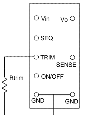
Figure 13. Circuit for Output Voltage Trim
