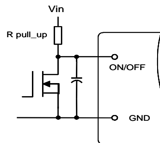
Figure 11. Circuit for Negative Logic Control
