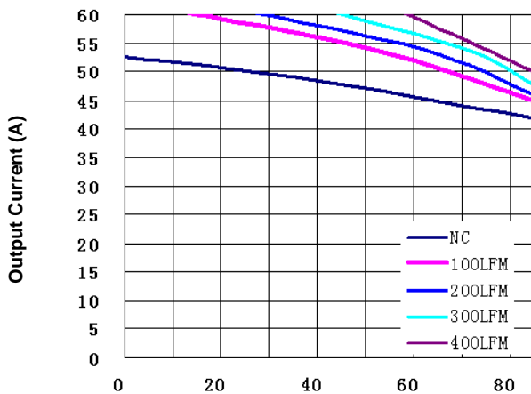
Figure 10a. Current Derating Curve (Vin=12V, Vo=0.8V, open frame)
