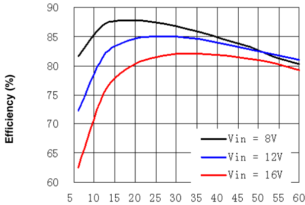
Figure 1a. Efficiency vs. Load Current (25°C, V_o=0.8V )
