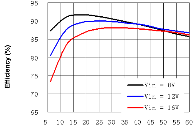
Figure 1d. Efficiency vs. Load Current (25°C, V_o=1.5V )
