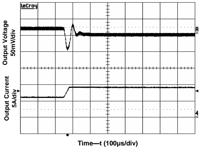
Figure 9. Transient Load Response Input voltage 12V, Output current 6A(50% full load), Slew rate 0.1A/µs
