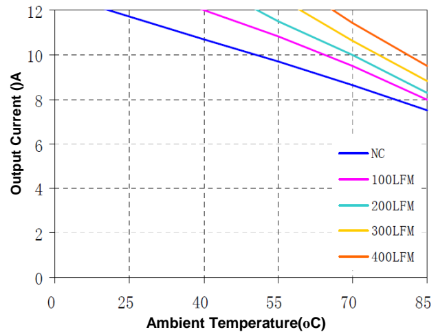
Figure 12(d). Current Derating Curve for 2.5V Output ( V_{in} = 12V open frame)
