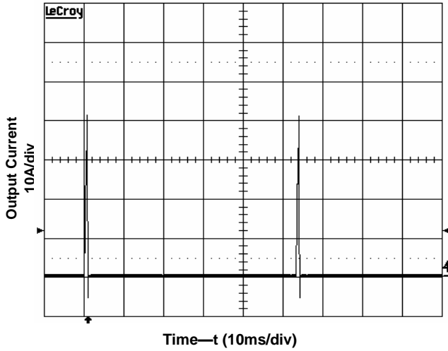
Figure 10. Short Circuit Current at Full Load
