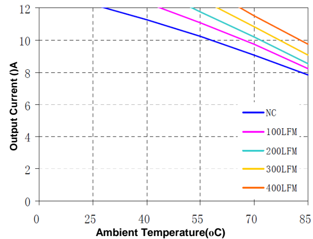
Figure 12(c). Current Derating Curve for 1.8V Output ( V_{in} = 12V open frame)
