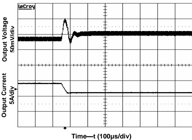
Figure 8. Transient Load Response Input voltage 12V, Output current 6A(50% full load), Slew rate 0.1A/µs.
