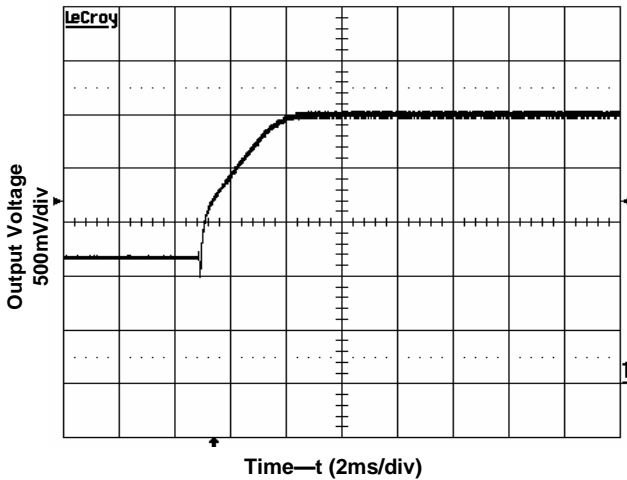
Figure 6. Start-Up with Prebias Input voltage 12V, Output current 0A, Output voltage 2.5V, Prebias 1.2V
