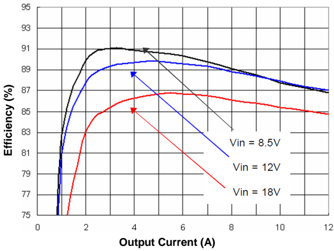
Figure 1(e). Efficiency vs. Load Current (25°C, 1.8V)
