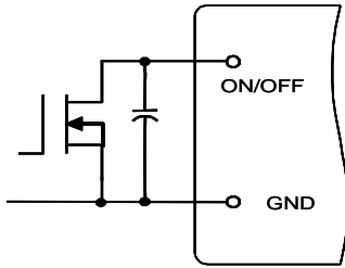
Fig. 13 Circuit for Positive Logic Control
