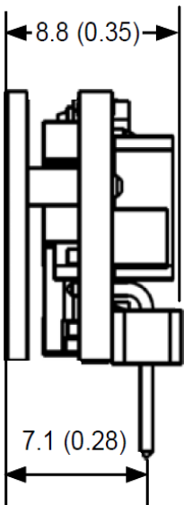
Side View with Baseplate
