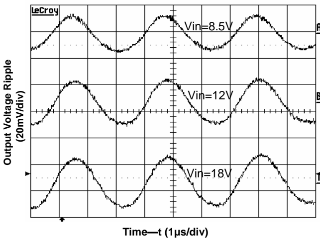
Figure 2. Output Ripple Voltage at 2.5V, 12A Output
