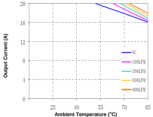
Figure 10b. Current Derating Curve (Vin=5V, Vo=1.2V, open frame)
