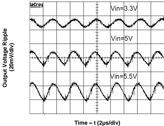
Figure 3. Output Ripple Voltage (1.0V/12A output)
