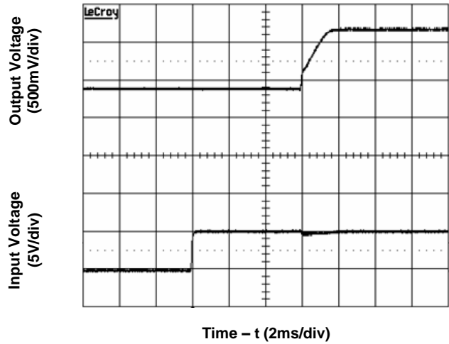
Figure 2. Start-Up with Pre-bias ( V_{in}=5V , 1.8V/0A output, pre-bias voltage=1.2V)
