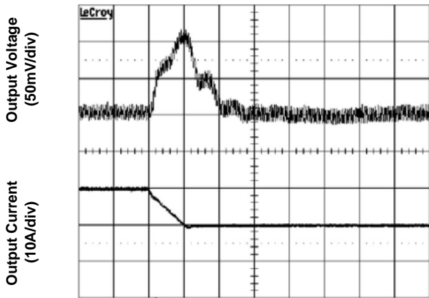
Time – t (50μs/div)
