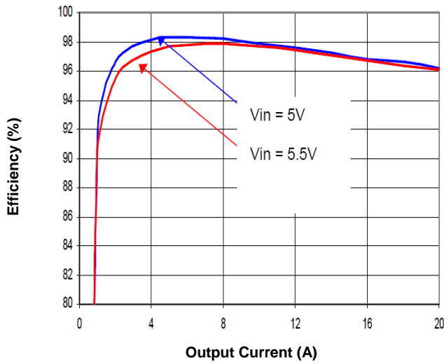
Figure 1g. Efficiency vs. Load Current (25°C, V_o=3.3V )
