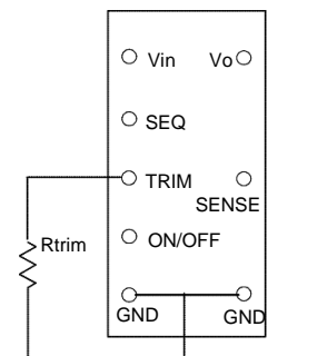
Figure 12. Circuit for Output Voltage Trim
