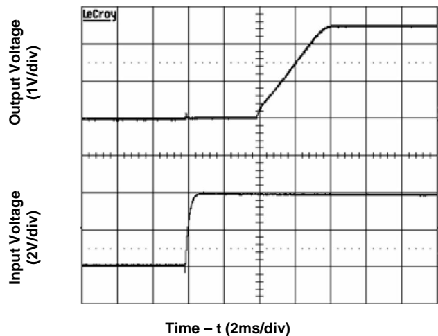
Figure 6. Start-Up from Application of Input Voltage ( V_{in}=4V , 2.5V/20A output)
