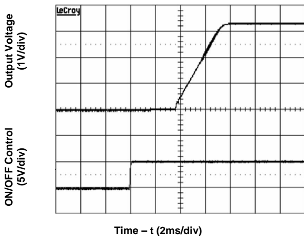
Figure 5. Start-Up from Enable Control ( V_{in}=5V , 3.3V/20A output)
