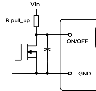
Figure 11. Circuit for Logic Control
