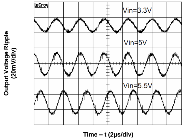
Figure 4. Output Ripple Voltage (2.5V/20A output)
