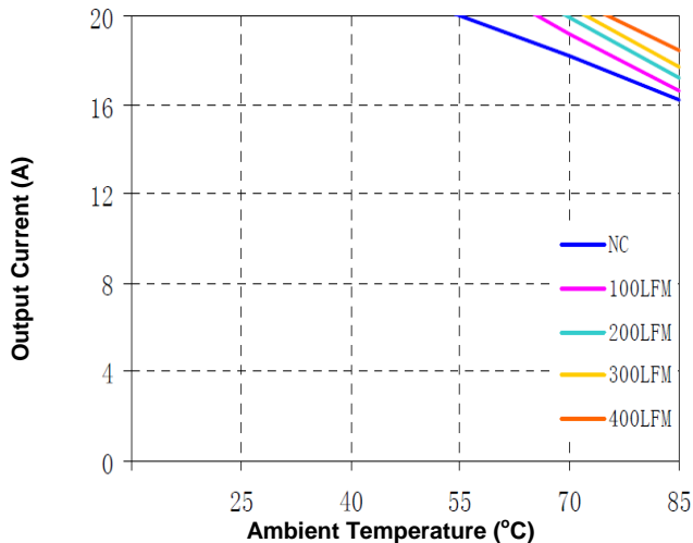
Figure 10a. Current Derating Curve (Vin=5V, Vo=1.0V, open frame)
