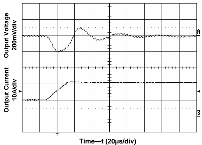
Figure 9. Transient Load Response Input voltage 12V, Output current 10A->20A, Slew rate 0.5A
