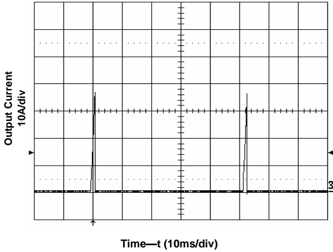
Figure 10 Short Circuit Current. V_{in} = 12V
