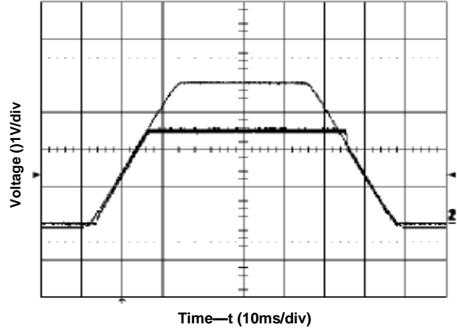
Figure 11 Voltage Tracking/Sequencing (with tracking option) V_{in} = 12V , V_o = 2.5V , I_o = 0A
