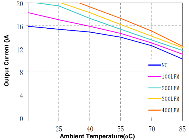
Figure 12(f) Current Derating Curve for 5.0V Output ( V_{in} = 12V_{open\ frame} )
