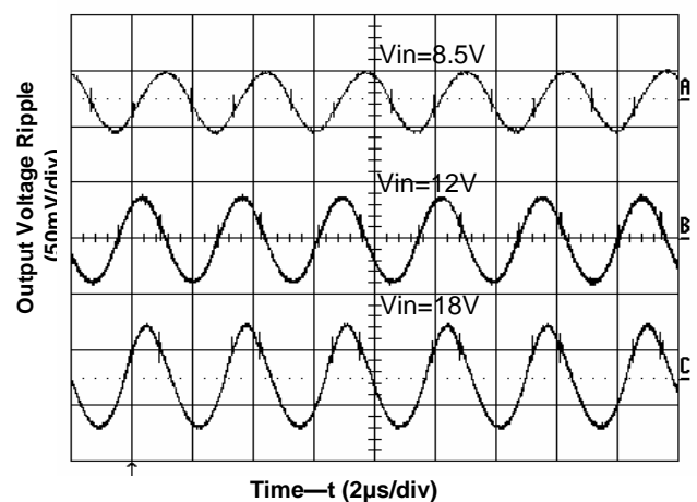
Figure 3. Output Reflected Ripple at 2.5V, 20A Output
