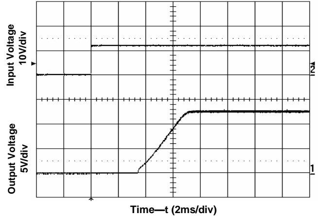
Figure 5. Start-up Application of Input Voltage Input voltage 12V, Output current 0A
