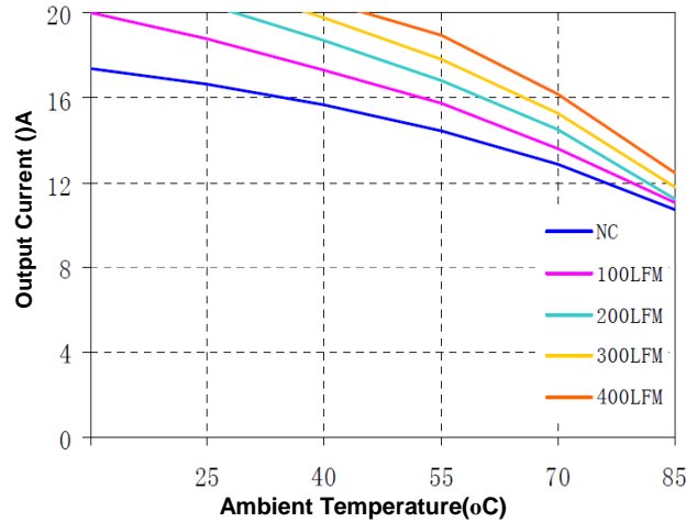
Figure 12(b) Current Derating Curve for 1.5V Output ( V_{in} = 12V open frame)
