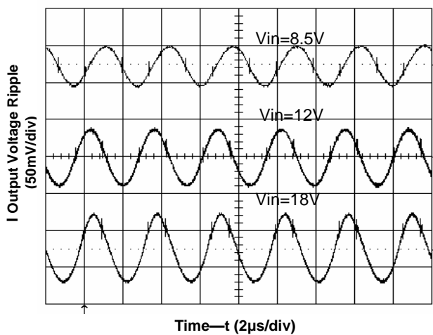
Figure 2. Output Voltage Ripple at 5V, 20A Output
