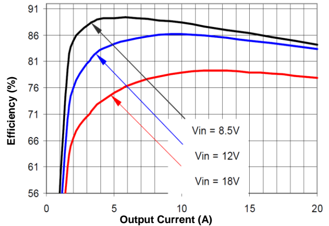
Figure 1(d). Efficiency vs. Load Current (25°C, 1.0V)
