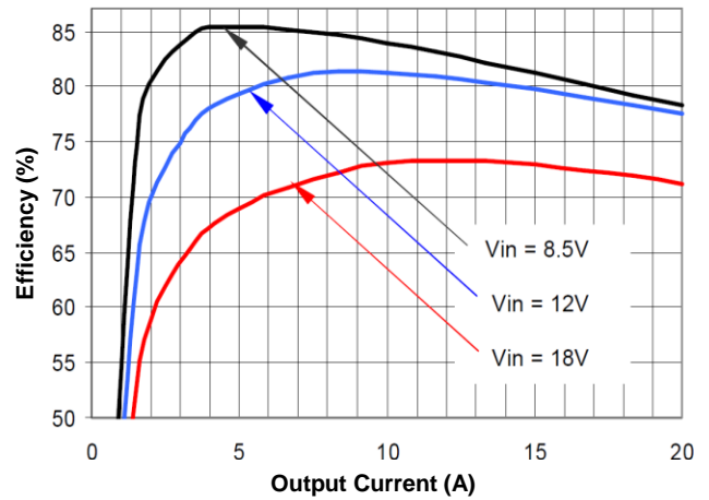
Figure 1(b). Efficiency vs. Load Current (25°C, 1V)
