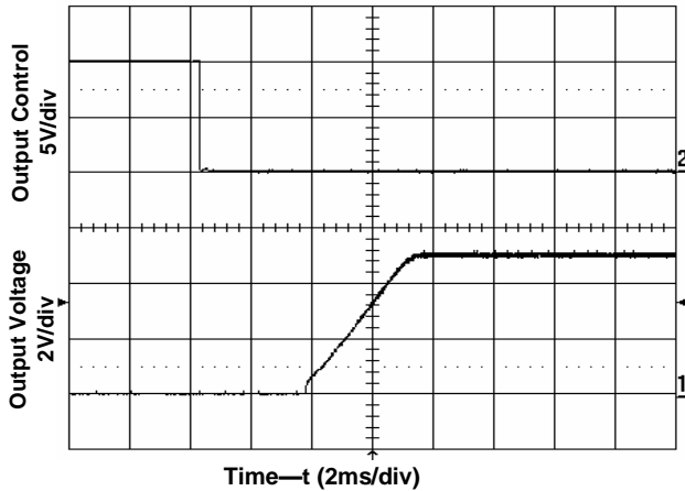
Figure 4. Start-Up from Enable Control Input voltage 12V, Output current 0
