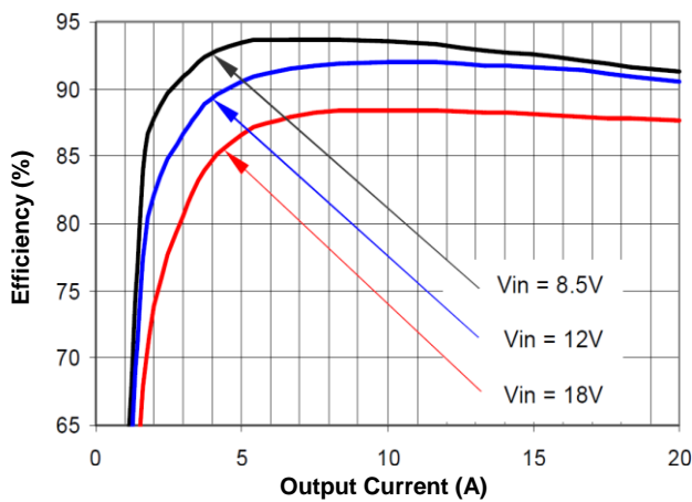
Figure 1(g). Efficiency vs. Load Current (25°C, 3.3V)
