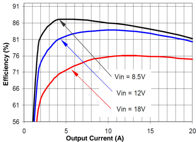
Figure 1(c). Efficiency vs. Load Current (25°C, 1.2V)
