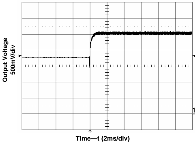
Figure 6. Start-Up with Prebias Input voltage 12V, Output current 0A, Output voltage 2.5V, Prebias 1.8V
