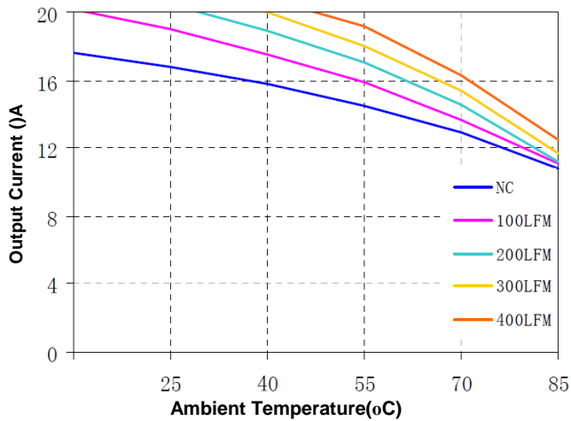
Figure 12(a) Current Derating Curve for 1.0V Output ( V_{in} = 12V open frame)
