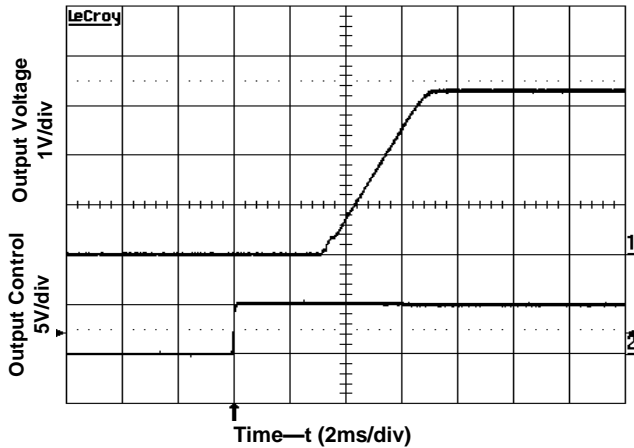
Figure 4. Start-Up from Enable Control Input voltage 5V, Output current 12A
