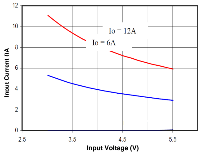
Figure 7 Input Characteristic (5V output)
