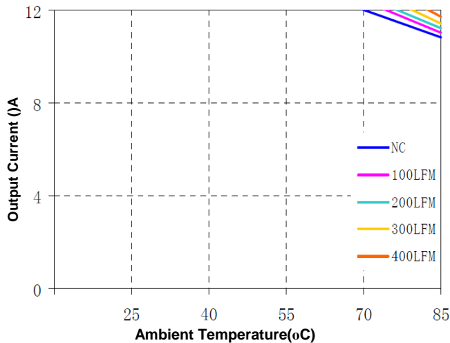
Figure 12(a) Current Derating Curve for 1.0V Output (Vin = 5V open frame)
