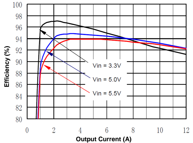
Figure 1(f). Efficiency vs. Load Current (25°C, 2.5V)
