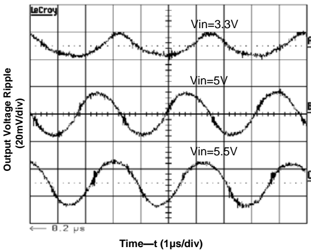
Figure 2. Output Voltage Ripple at 2.5V, 12A Output
