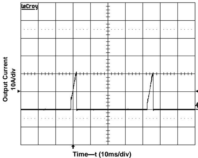
Figure 10 Short Circuit Current. Vin = 5V
