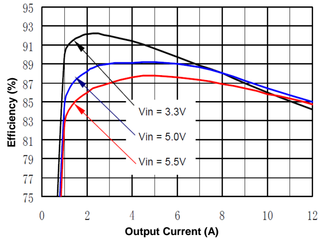
Figure 1(b). Efficiency vs. Load Current (25°C, 1V)
