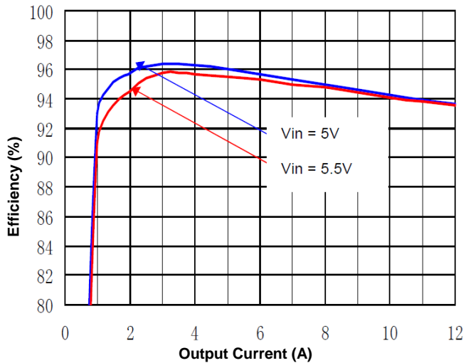
Figure 1(g). Efficiency vs. Load Current (25°C, 3.3V)
