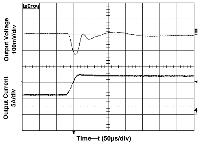
Figure 9 Transient Load Response Input voltage 5V, Output current 6A(50% full load), Slew rate 0.2A/µs
