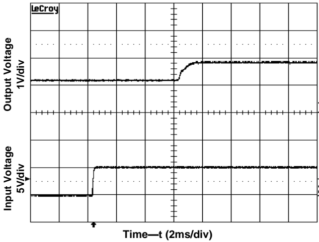
Figure 6. Start-Up with Prebias Input voltage 5V, Output current 0A, Output voltage 1.8V, Prebias 1.2V
