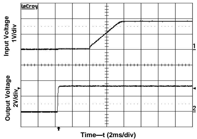
Figure 5. Start-up Application of Input Voltage Input voltage 3.3V, Output current 12A
