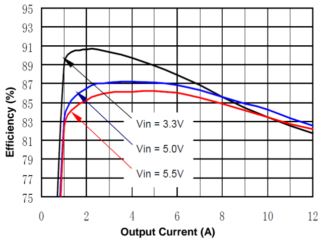
Figure 1(a). Efficiency vs. Load Current (25°C, 0.8V)
