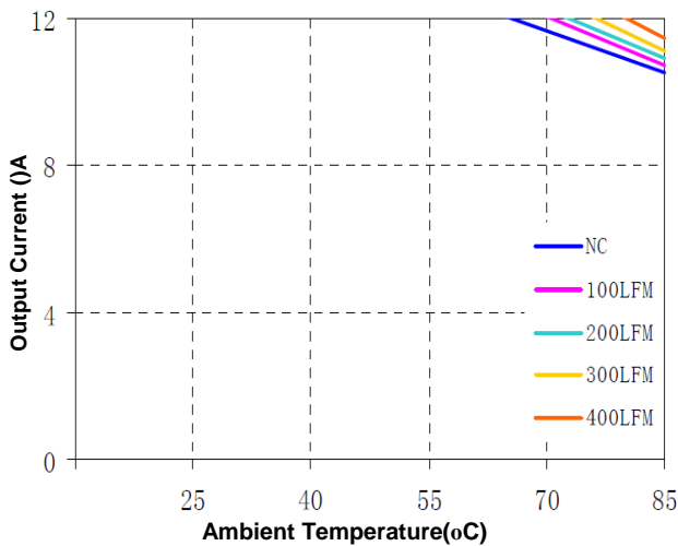
Figure 12(c) Current Derating Curve for 1.5V Output (Vin = 5V open frame)
