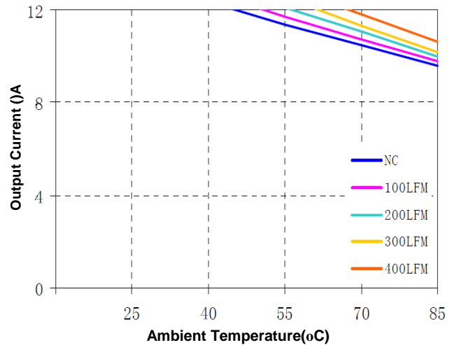
Figure 12(f) Current Derating Curve for 3.3V Output ( V_{in} = 5V_{open\ frame} )
