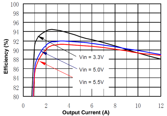
Figure 1(d). Efficiency vs. Load Current (25°C, 1.5V)
