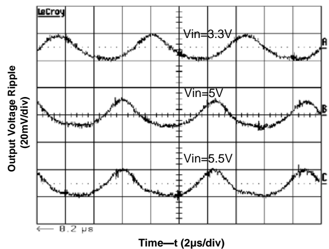
Figure 3. Output Voltage Ripple at 1V, 12A Output
