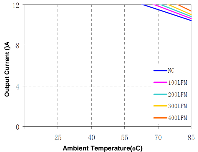
Figure 12(b) Current Derating Curve for 1.2V Output (Vin = 5V open frame)
