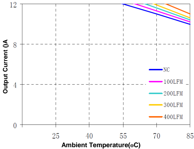
Figure 12(e) Current Derating Curve for 2.5V Output ( V_{in} = 5V_{open\ frame} )
