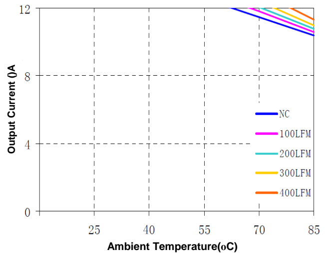
Figure 12(d) Current Derating Curve for 1.8V Output (Vin = 5V open frame)
