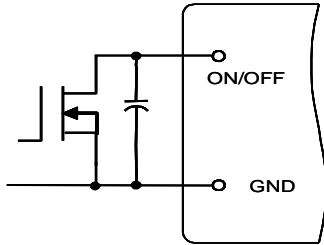
Fig. 13 Circuit for Positive Logic Control
