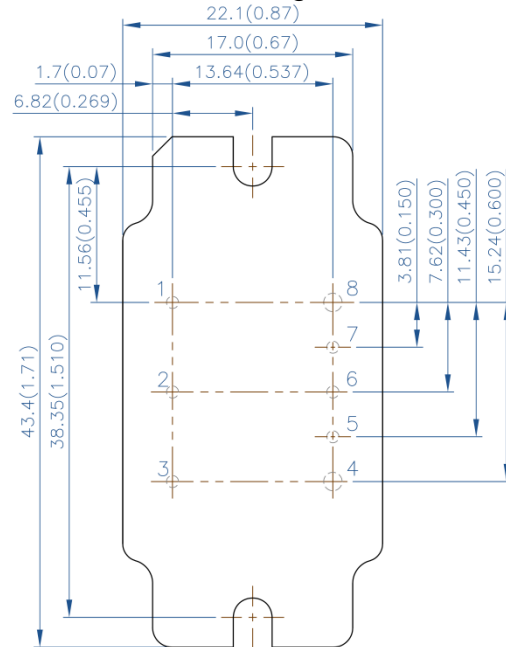
With flange
