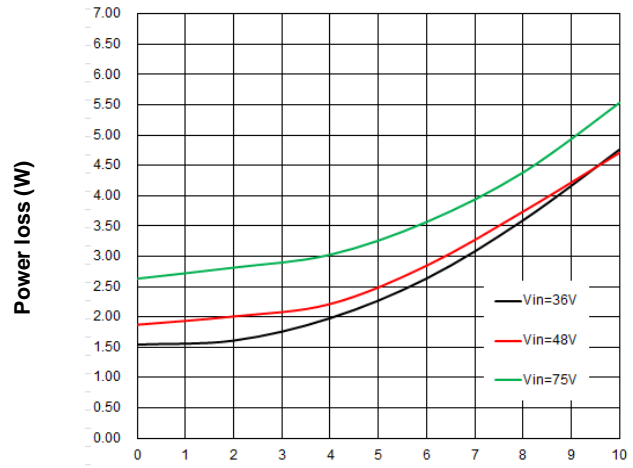
Figure 2. Power loss vs. Output Current (25°C)
