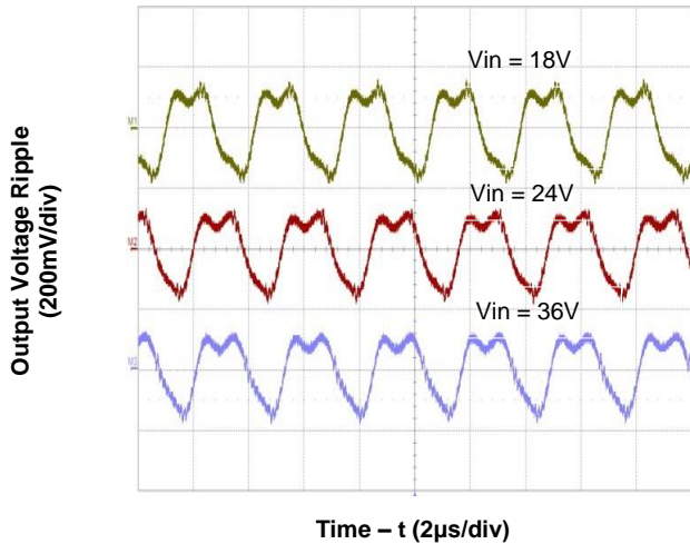
Figure 3. Output Voltage Ripple at Full Load (Tested with 4x4.7µF ceramic output capacitor)
