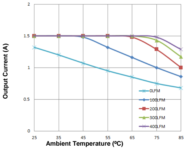
Figure 7. Current Derating Curve with Open Frame (Direction 3 (Ref. Figure 8); typical Vin, soldered interface)
