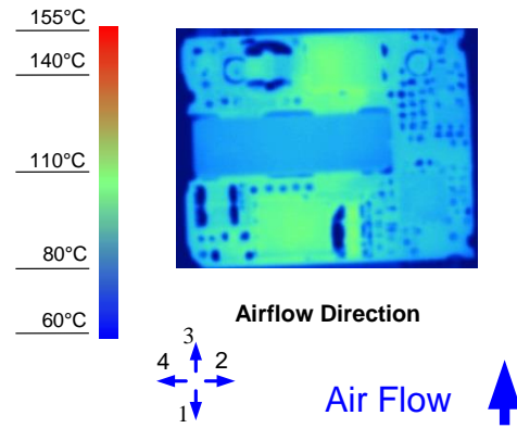
Figure 8. Thermal Image for Airflow Direction 3 (1.5A output, 55°C ambient, 200 LFM, typical Vin, open frame unit)
