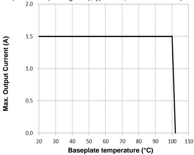
Figure 9. Current Derating Curve for Baseplate (typical vin with baseplate; solder interface)
