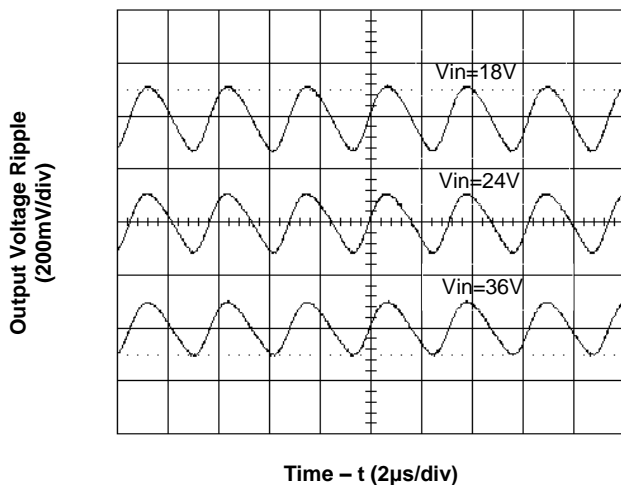
Figure 5. Output Voltage Ripple at Full Load (tested with no external output capacitor)
