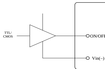
Figure 14. Direct Logic Drive
