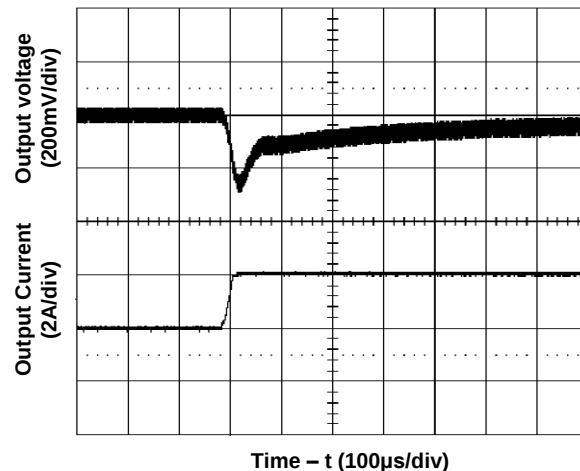
Figure 8. Transient Load Response
