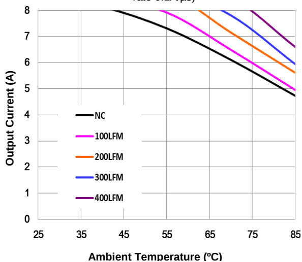
Figure 9. Current Derating Curve with Open Frame (Direction 3 (Ref. Figure 10); typical Vin, soldered interface)
