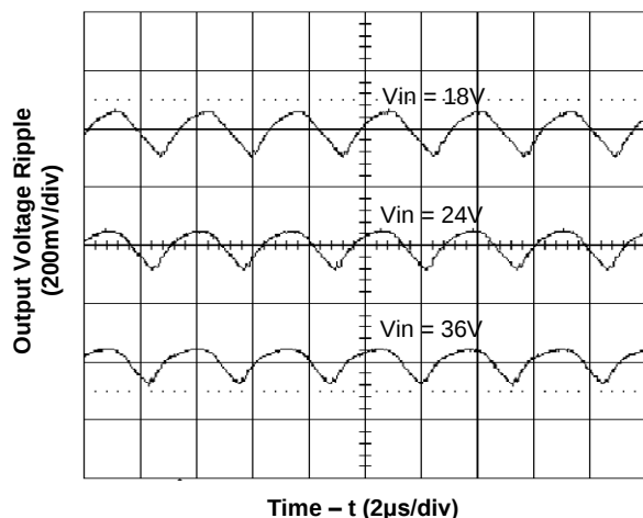
Figure 5. Output Voltage Ripple at Full Load (tested with no ceramic output capacitor)
