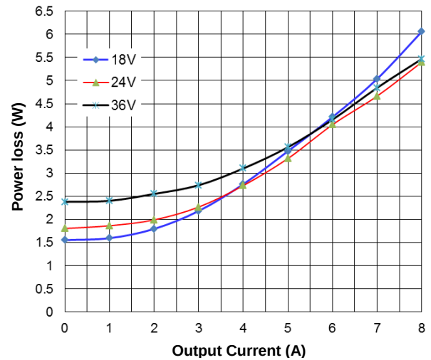
Figure 2. Power loss vs. Output Current (25°C)
