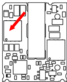
Figure 17. Temperature Monitoring Locations
