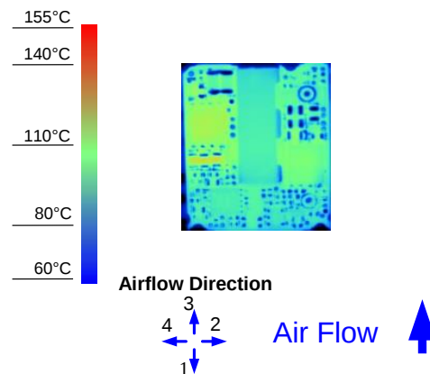
Figure 10. Thermal Image for Airflow Direction 3 (8A output, 55°C ambient, 200 LFM, typical Vin, open frame)
