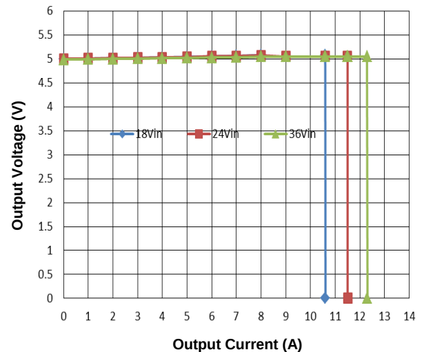
Figure 4. Output Characteristics
