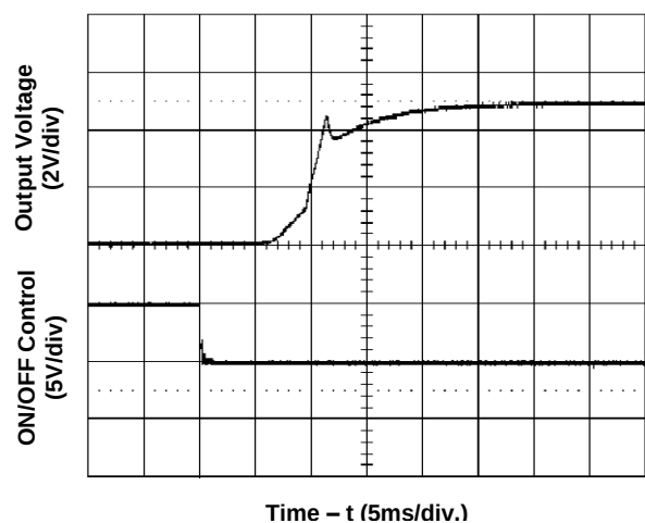
Figure 6. Start-Up from Enable Control (typical Vin, full load, no external output capacitor)
