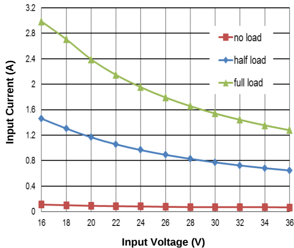
Figure 3. Input Characteristics
