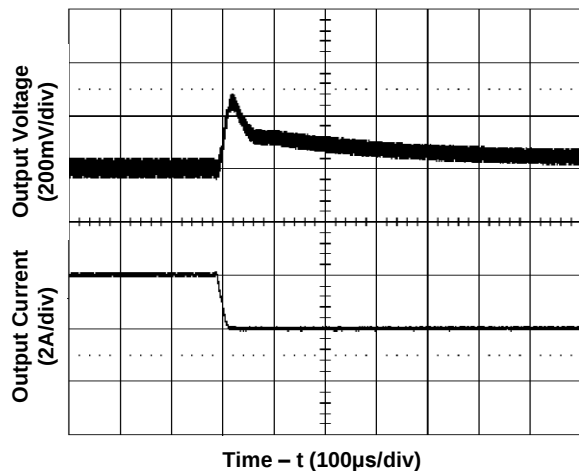
Figure 7. Transient Load Response
