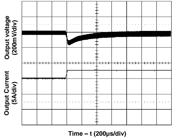
Figure 8. Transient Load Response (typical Vin, load current steps from 50% to 75% at a slew rate 0.1A/µs, tested with 400µF external output capacitor)
