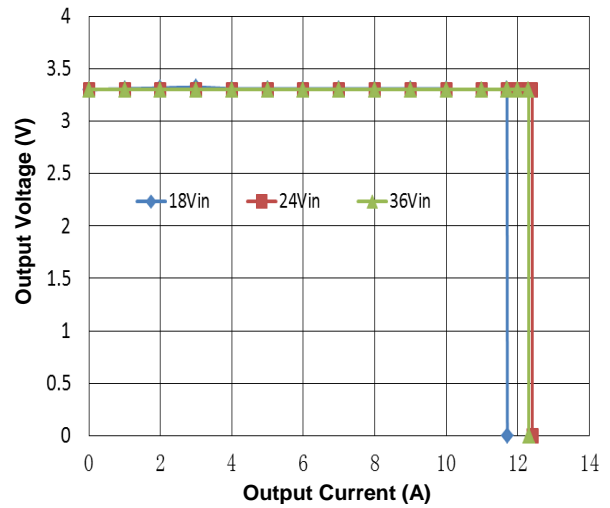
Figure 4. Output Characteristics (25°C)
