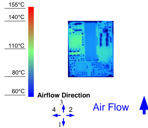
Figure 10. Thermal Image for Airflow Direction 3 (10A output, 55°C ambient, 200 LFM, typical Vin, Open frame unit)
