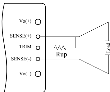
Figure 16. Circuit to Increase Output Voltage
