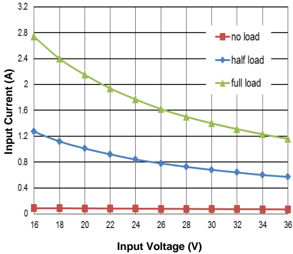
Figure 3. Input Characteristics (25°C)
