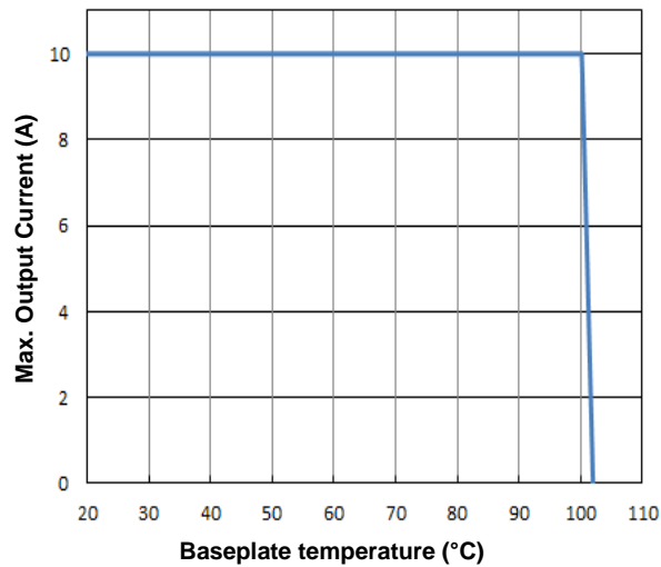
Figure 11. Current Derating Curve for Baseplate (typical Vin with baseplate; soldered interface)
