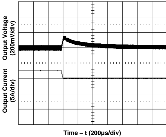
Figure 7. Transient Load Response (typical Vin, load current steps from 75% to 50% at a slew rate 0.1A/µs, tested with 400µF external output capacitor)
