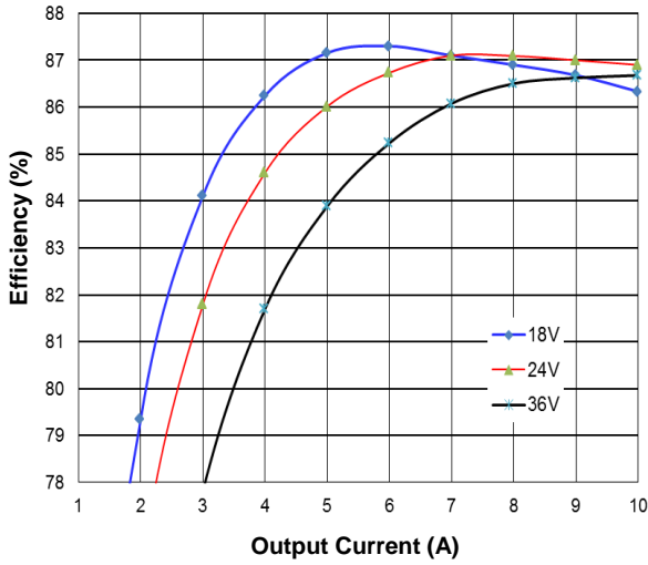
Figure 1. Efficiency vs. Load Current (25°C)
