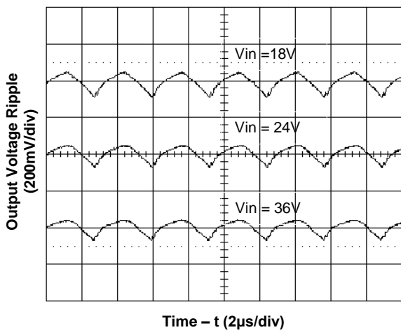
Figure 5. Output Ripple Voltage at Full Load (tested with no external output capacitor)
