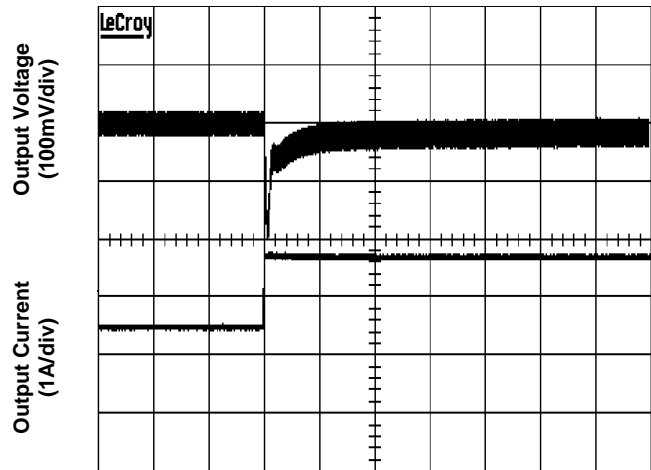
Time - t (500μs/div) Figure 8. Transient Load Response (typical Vin, load current steps from 50% to 75% at a slew rate 0.1A/μs)
