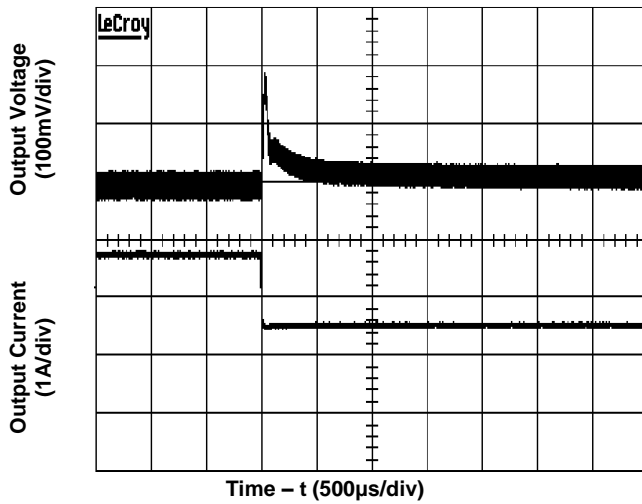
Time - t (500μs/div) Figure 7. Transient Load Response (typical Vin, load current steps from 75% to 50% at a slew rate 0.1A/μs)
