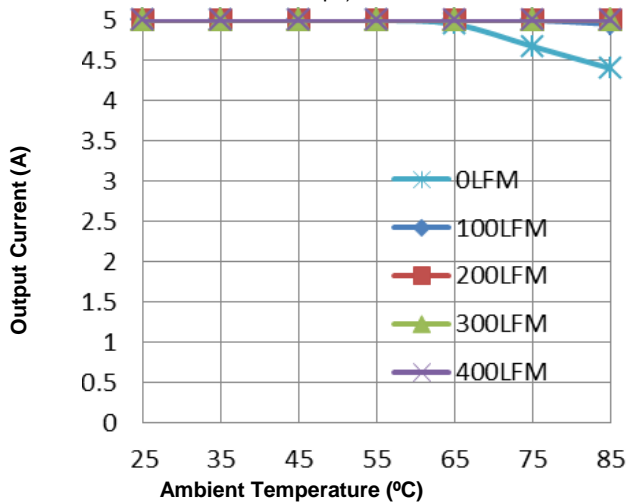
Figure 9. Current Derating Curve with Open Frame (Direction 3 (Ref. Figure 10); typical Vin, soldered interface)
