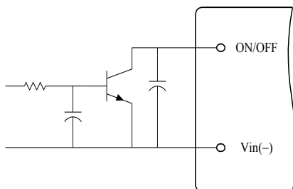
Figure 12. Opto Coupler Enable Circuit
