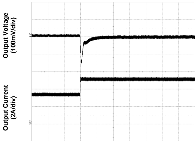
Time - t (500µs/div) Figure 8. Transient Load Response
