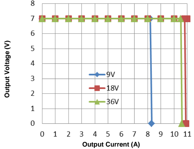
Figure 4. Output Characteristic
