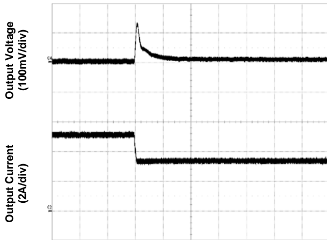
Time - t (500µs/div) Figure 7. Transient Load Response
