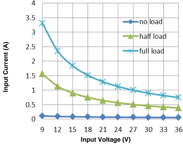
Figure 3. Input Characteristic
