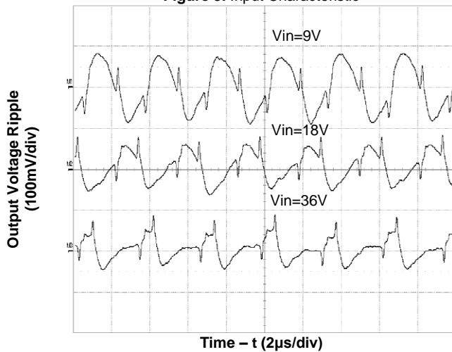
Figure 5. Output Ripple Voltage at Full Load (tested with 4x47µF ceramic output capacitors)
