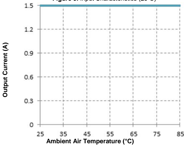
Figure 11. Current Derating Curve under Nature Convection (Ref. Fig. 12 for Airflow Direction; typical V_{in} , open frame unit, soldered interface)
