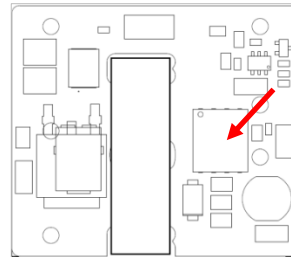
Figure 18. Temperature Monitoring Locations
