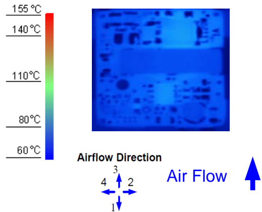
Figure 12. Thermal Image for Airflow Direction 3 (1.5A output, 55°C ambient, 200 LFM, typical V_{in} open frame unit, soldered interface)
