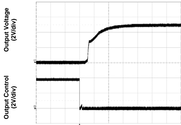
Figure 4. Start-Up from Enable Control (typical Vin and full load)
