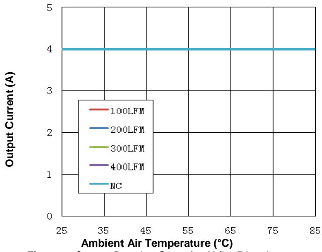
Figure 7. Current Derating Curve for AirflowDirection3 (Ref. Fig. 8 for Airflow Direction; typical Vin, open frame unit, soldered interface)
