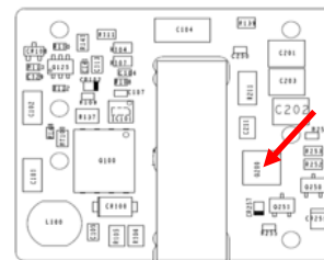
Figure 14. Temperature Monitoring Locations
