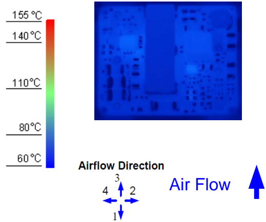
Figure 8. Thermal Image for Airflow Direction 3 (4A output, 55°C ambient, 200 LFM, typical Vin open frame unit, soldered interface)
