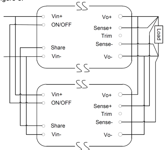
Figure 6. Circuit Configuration for Active Current Sharing
