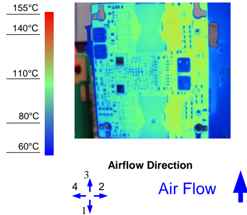
Figure 8. Thermal Image for Airflow Direction 3 (39A output, 55°C ambient, 200 LFM, typical Vin, open frame unit)
