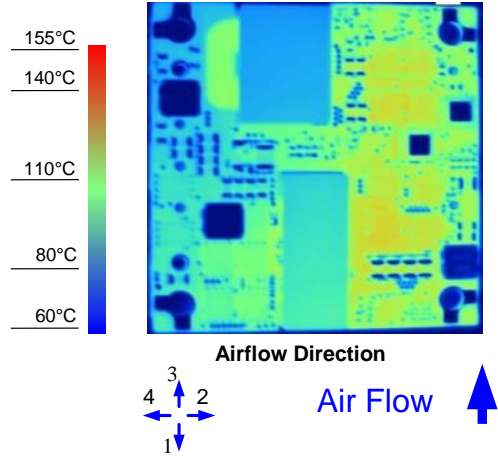
Figure 8. Thermal Image for Airflow Direction 3 (25.5A output, 55°C ambient, 200 LFM, typical Vin, open frame, unit soldered onto a fixture board)
