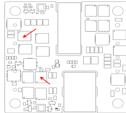
Figure 16. Temperature Monitoring Location
