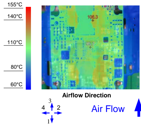
Figure 8. Thermal Image for Airflow Direction 3 (9A output, 55°C ambient, 200 LFM, typical Vin, open frame unit)
