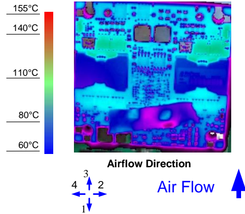
Figure 8. Thermal Image for Airflow Direction 3 (12A output, 55°C ambient, 200 LFM, typical Vin, open frame unit)
