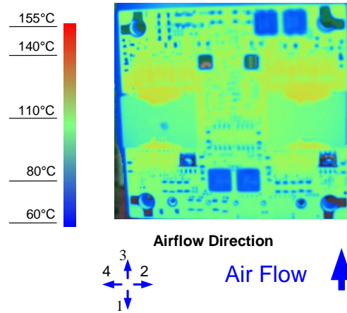
Figure 8. Thermal Image for Airflow Direction 3 (15A output, 55°C ambient, 200 LFM, typical Vin, open frame unit)
