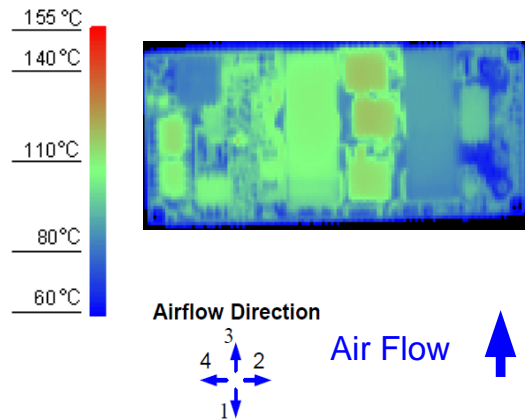
Figure 12. Thermal Image for Airflow Direction 3 (40A output, 55°C ambient, 200 LFM, typical Vin, open frame, socket interface)
