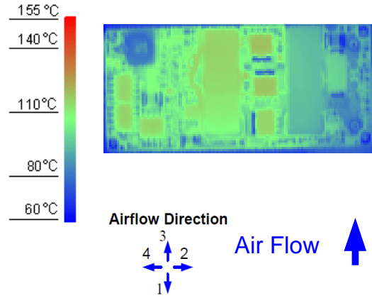
Figure 10. Thermal Image for Airflow Direction 3 (35A output, 55°C ambient, 200 LFM, typical Vin, open frame, socket interface)
