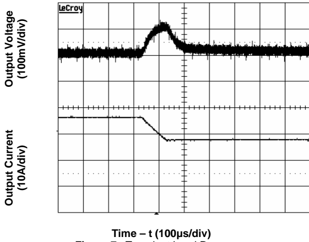
Figure 7. Transient Load Response (typical Vin, load current steps from 50% to 25% at a slew rate 0.1A/µs)
