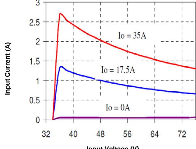
Figure 4. Input Characteristics (25°C)
