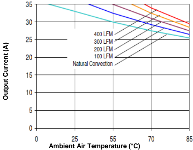
Figure 9. Current Derating Curve for Airflow Direction 3 (Ref. Fig. 10 for Airflow Direction; Vin = 48V, open frame)
