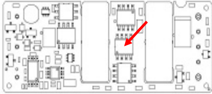
Figure 16. Temperature Monitoring Locations
