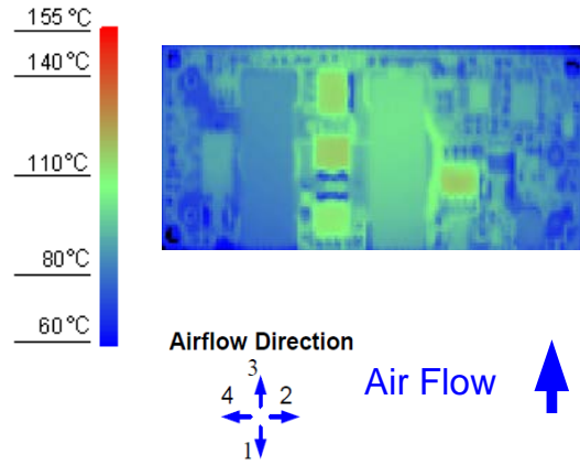
Figure 10. Thermal Image for Airflow Direction 3 (40A output, 55°C ambient, 200 LFM, typical Vin, open frame, socket interface)
