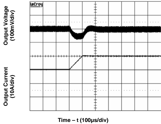
Figure 8. Transient Load Response (typical Vin, load current steps from 50% to 75% at a slew rate 0.1A/µs)
