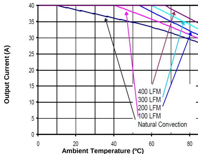
Figure 7. Current Derating Curve with Open Frame (Direction 3 (Ref. Figure 8); typical Vin)
