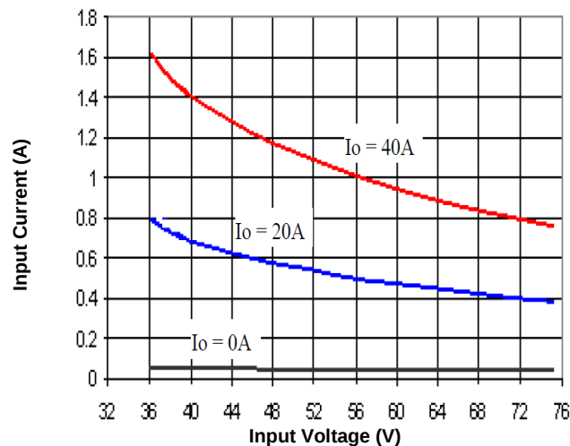
Figure 2. Input Characteristics (25°C)
