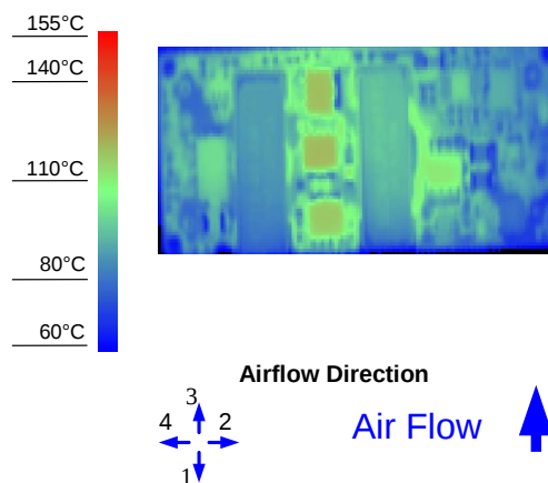
Figure 8. Thermal Image for Airflow Direction 3 (27.5A output, 55°C ambient, 200 LFM, typical Vin, open frame unit)
