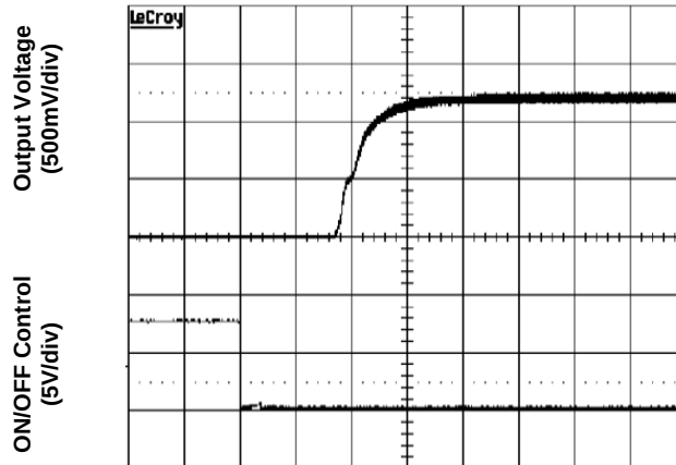
Figure 4. Start-Up from Enable Control (typical V_{in} , zero load)
