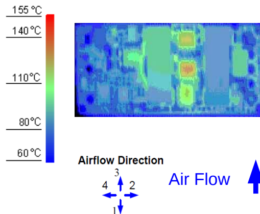
Figure 12. Thermal Image for Airflow Direction 3 (27.5A output, 55°C ambient, 200 LFM, typical Vin, open frame, socket interface)
