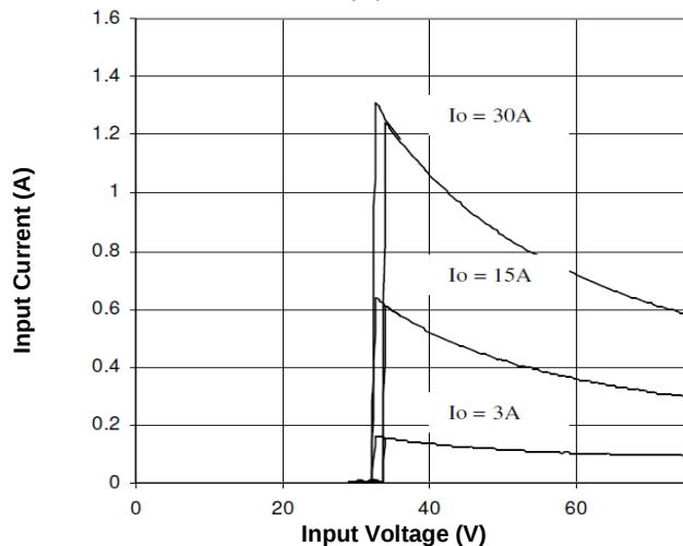
Figure 9. Input Characteristics
