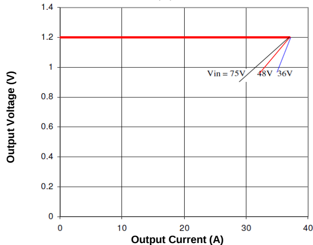
Figure 10. Output Characteristics
