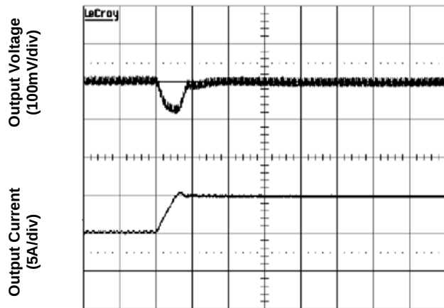
Figure 7. Transient Load Response
