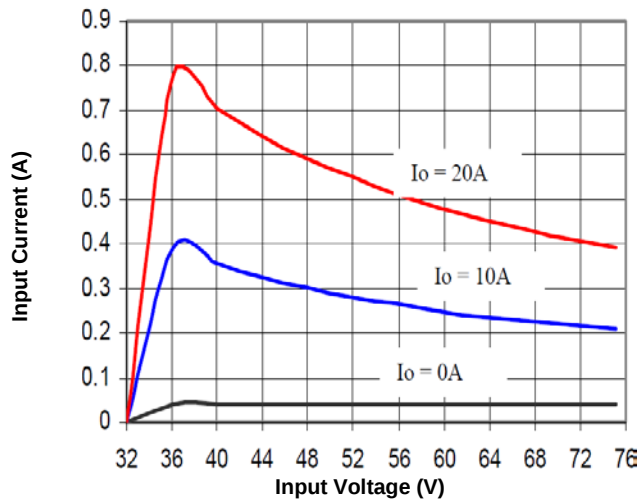
Figure 9. Input Characteristics
