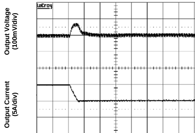
Figure 8. Transient Load Response
