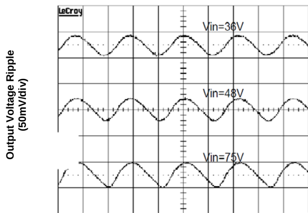
Figure 5. Output Ripple Voltage at Full Load
