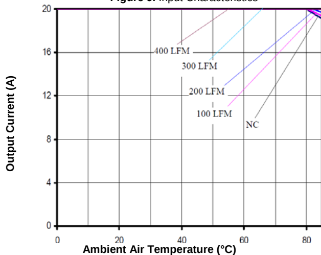
Figure 11. Current Derating Curve for Airflow Direction 3 (Ref. Fig. 12 for Airflow Direction; V_{in} = 36V, open frame)
