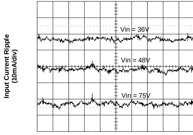
Figure 6. Input Reflected Ripple Current at Full Load
