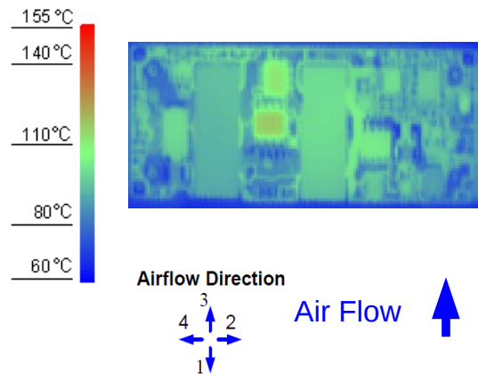
Figure 12. Thermal Image for Airflow Direction 3 (19.1A output, 55°C ambient, 200 LFM, typical V_{in} , open frame, socket interface)
