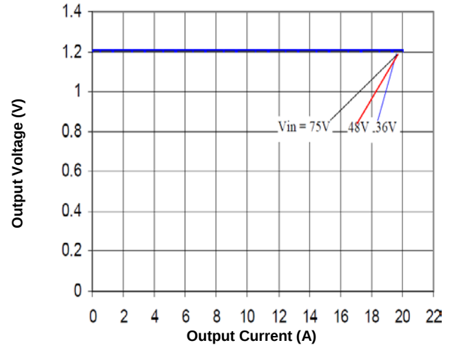
Figure 10. Output Characteristics
