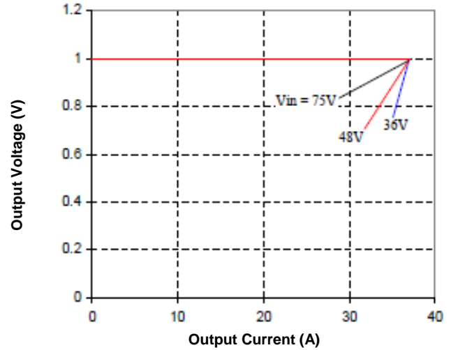
Figure 10. Output Characteristics
