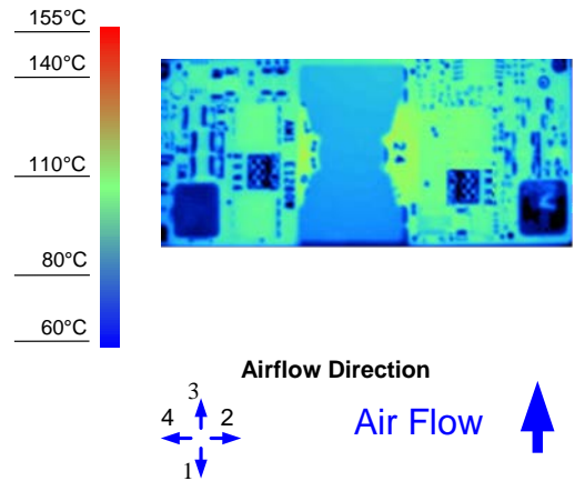
Figure 8. Thermal Image for Airflow Direction 3 (3A output, 55°C ambient, 200 LFM, typical Vin, open frame)
