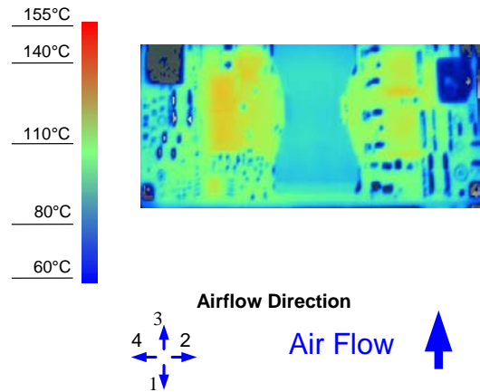
Figure 8. Thermal Image for Airflow Direction 3 (6A output, 55°C ambient, 200 LFM, typical Vin, open frame, unit soldered onto a fixture board)
