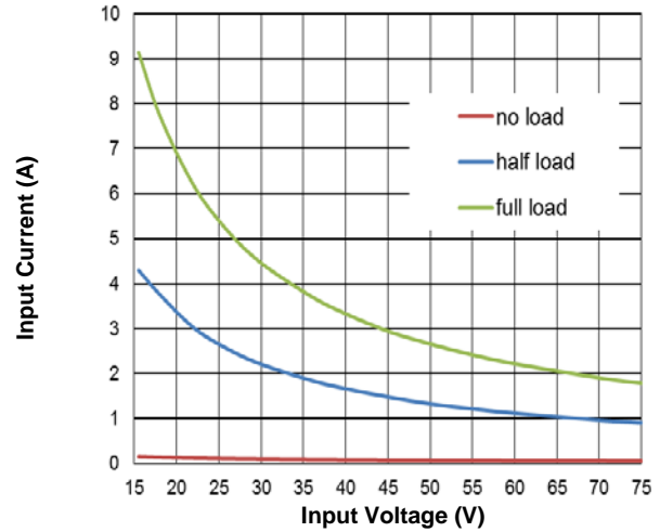
Figure 2. Input Characteristics (25°C)
