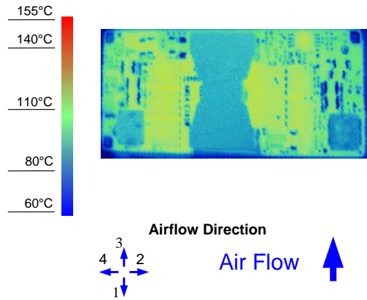
Figure 8. Thermal Image for Airflow Direction 3 (13.2A output, 55°C ambient, 200 LFM, typical Vin, open frame, unit soldered onto a fixture board)
