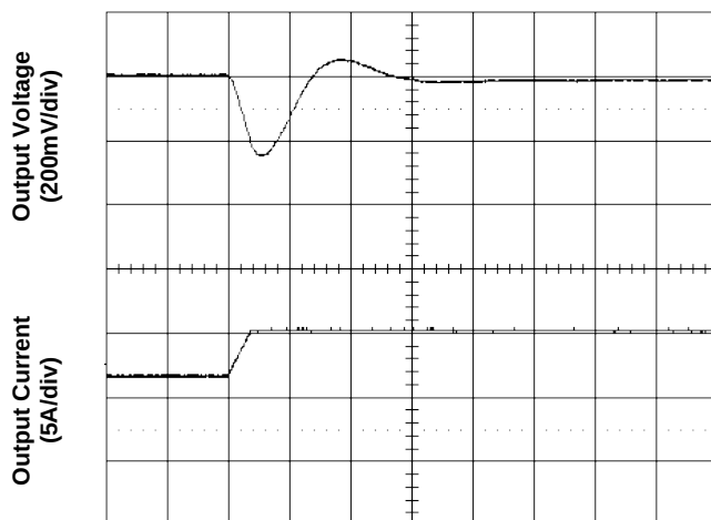
Figure 8. Transient Load Response (typical V_{in} , load current steps from 50% to 75% at a slew rate 0.1A/\mu s )
