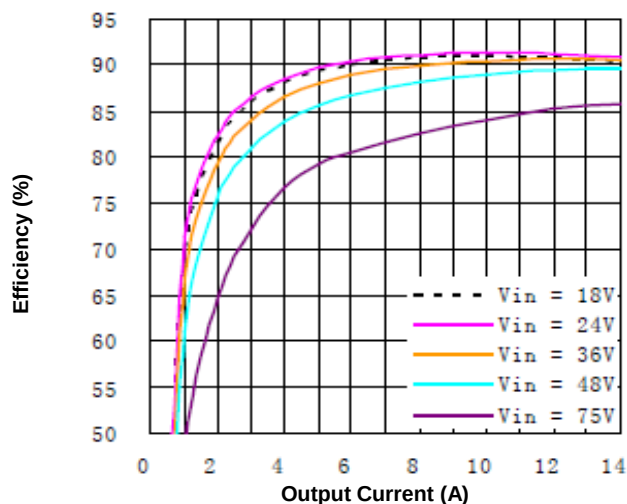
Figure 1. Efficiency vs. Load Current (25°C)
