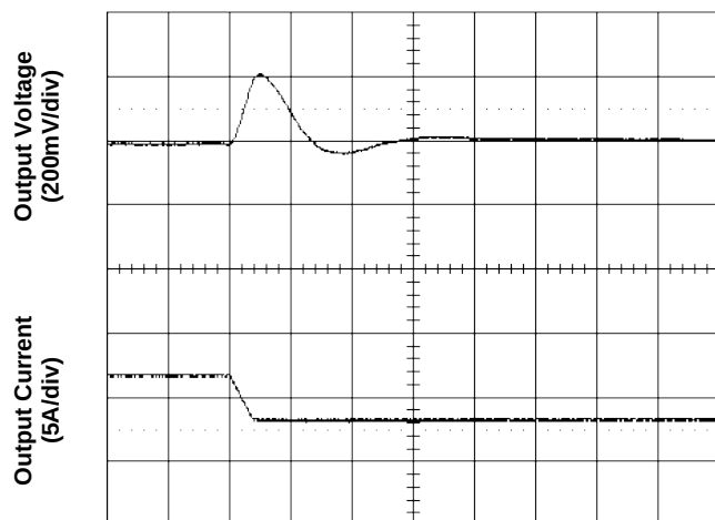
Figure 7. Transient Load Response (typical V_{in} , load current steps from 50% to 25% at a slew rate 0.1A/\mu s )
