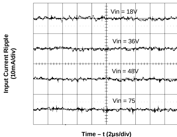
Figure 6. Input Reflected Ripple Current at Full Load
