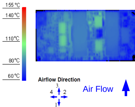
Figure 12. Thermal Image for Airflow Direction 3 (14A output, 55°C ambient, 200 LFM, typical V_{in} open frame unit)
