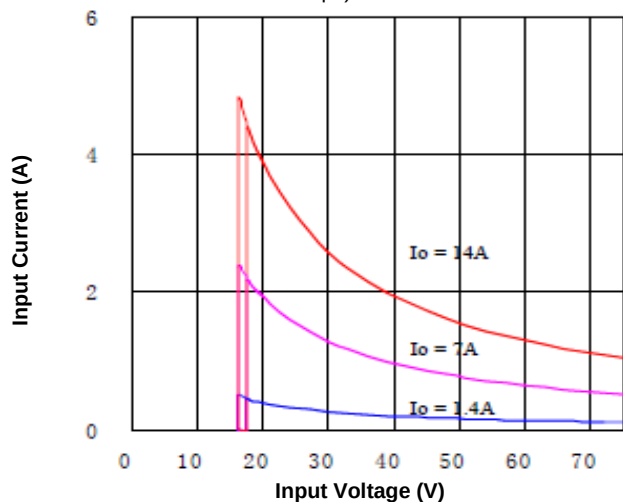
Figure 9. Input Characteristics (25°C)
