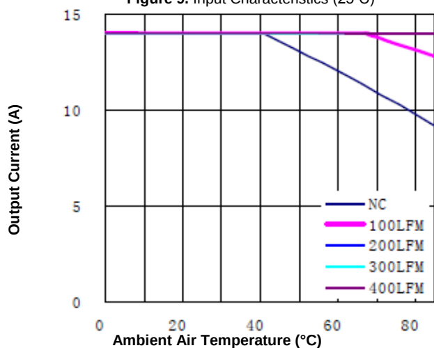
Figure 11. Current Derating Curve for Airflow Direction 3 (Ref. Fig. 12 for Airflow Direction; V_{in} = 36V , open frame unit using solder interface)
