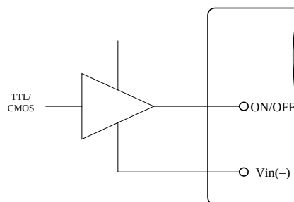
Figure 15. Direct Logic Drive
