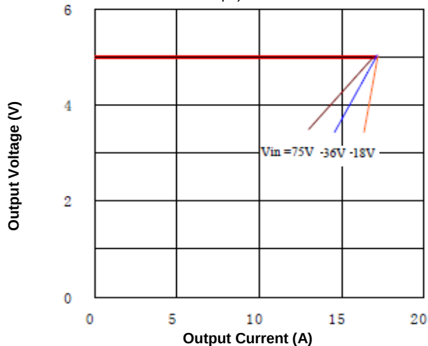
Figure 10. Output Characteristics (25°C)
