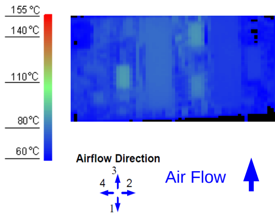
Figure 12. Thermal Image for Airflow Direction 3 (9A output, 55°C ambient, 200 LFM, typical Vin open frame unit)
