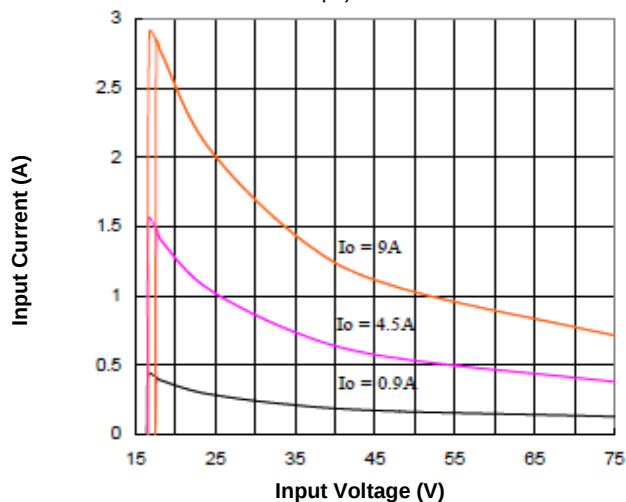
Figure 9. Input Characteristics (25°C)
