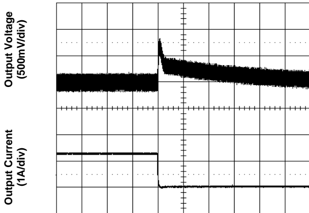
Figure 7. Transient Load Response (typical V_{in} , load current steps from 50% to 25% at a slew rate 0.1A/μs)
