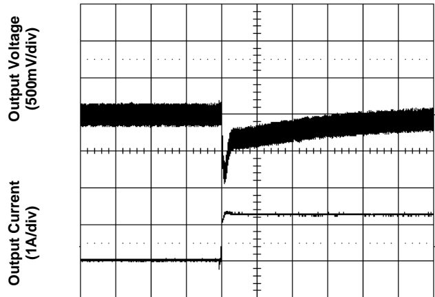
Figure 8. Transient Load Response (typical V_{in} , load current steps from 50% to 75% at a slew rate 0.1A/μs)
