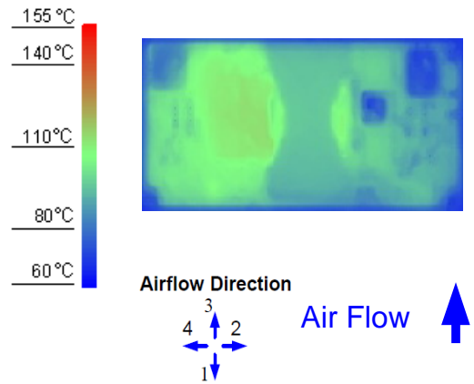
Figure 12. Thermal Image for Airflow Direction 3 (4.6A output, 55°C ambient, 200 LFM, V_{in} = 24V open frame unit)
