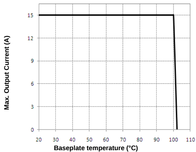
Figure 13. Current Derating Curve for Baseplate (typical V_{in} with baseplate; solder interface)
