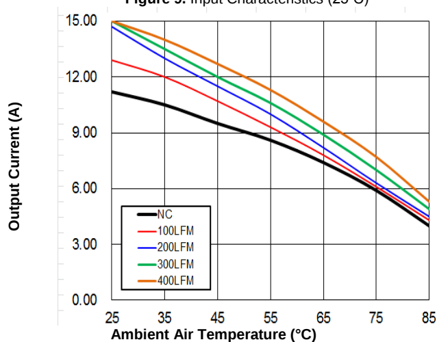
Figure 11. Current Derating Curve for Airflow Direction 3
