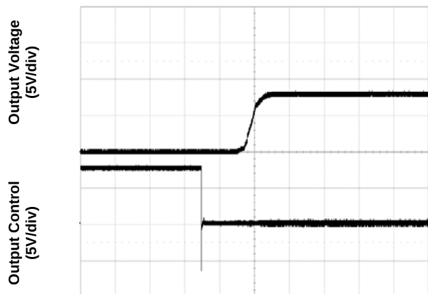
Figure 3. Start-Up from Enable Control (typical V_{in} and full load)
