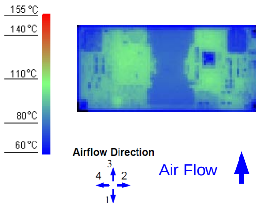
Figure 12. Thermal Image for Airflow Direction 3 (13A output, 55°C ambient, 200 LFM, Vin = 24V open frame unit)
